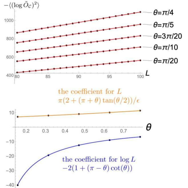
FIG. 2: The numerical results of -\langle(\log \tilde{O}_{\mathcal{C}})^2\rangle (in the unit of \sigma\pi^2/N^2 ) for the shape in FIG. 1 with different angles. The UV cut-off is set to be \epsilon = 1 . The large- L scaling is fitted by the function -\langle(\log \tilde{O}_{\mathcal{C}})^2\rangle = aL/\epsilon + b \log L + c/L + d , and the fitting parameters a, b agree with the analytical expressions Eq. 13 and Eq. 14.
