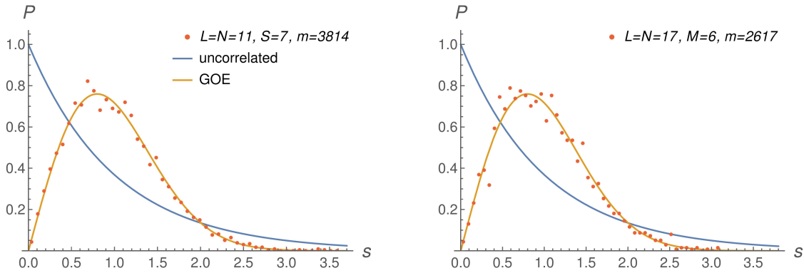
Figure 3: Distribution of spacings for different sectors of \mathcal{N} = 4 SYM at N = L , against the GOE distribution. On the left we consider the \mathfrak{sl}(2) sector, and on the right we have the \mathfrak{su}(2) sector. In both cases we focus on the positive parity sector, and clip 11% and 4% of low- and high-energy states respectively.
