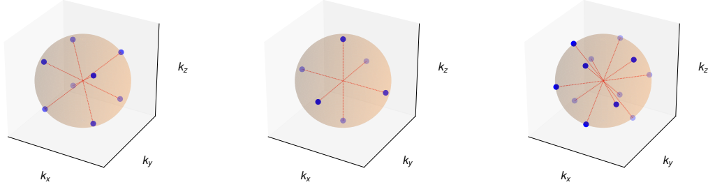
Figure 4: Gapless nodes in the Bogoliubov quasiparticle dispersions for odd-parity order parameters formed by fermions belonging to j = 1/2 or j = 3/2 sectors independently. (a): Gapless nodes for T_{+(1,2,3)}^{J=1,3}, T_2^{J=3} order parameters resulting from two-channel Kondo interaction are located along body diagonal [111] directions. (b): Gapless nodes for T_{-(1,2,3)}^{J=1,3} order parameters resulting from two-channel Kondo interaction are located along primary cubic \hat{e}_i axes. (c): Gapless nodes for T_{+;j=3/2}^{J=1,3}, T_{-;j=3/2}^{J=1,3}, T_{2;j=3/2}^{J=3} resulting from novel Kondo interaction are located along the [1 \pm 10], [10 \pm 1], [01 \pm 1] axes. The red-dashed lines are for ease of viewing the directions of gapless points.
