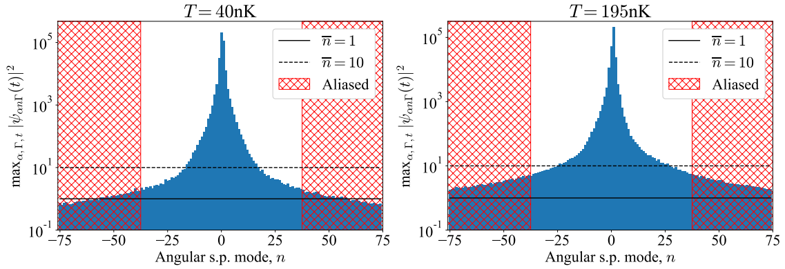
Figure 13: Maximum average occupation of the angular single-particle modes with a given n index, in simulations of the full experimental sequence for temperatures T = 40\text{nK} and T = 195\text{nK} , with respective barrier heights V_b = 0.78\mu and V_b = 0.67\mu . For a grid with n_\theta = 150 points, modes in the red hatched region are formally subject to aliasing. The aliased modes have a maximum occupation on the order of 1, and are never occupied by 10 or more atoms.
