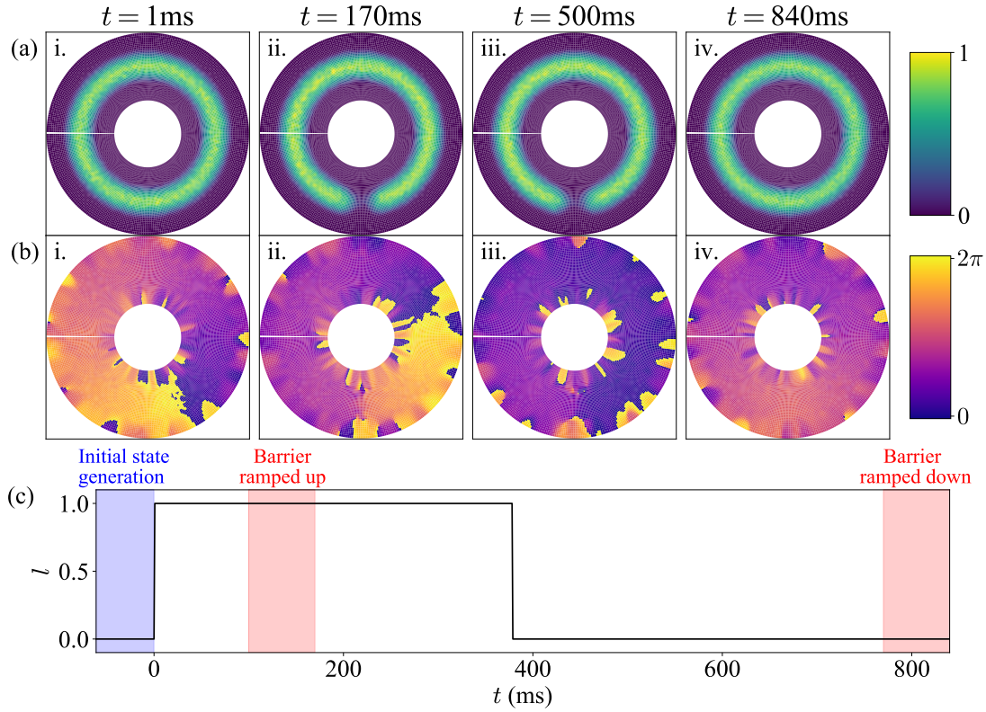
Figure 4: Single trajectory of the SPGPE for a simulation of the experimental sequence at T = 85\text{nK} with the barrier held at its maximum strength V_b = 0.82\mu for t_{\text{hold}} = 600\text{ms} . Slices of the density normalised to 1 and phase in the x - y plane are shown in (a) and (b), respectively, at different times. The winding number as a function of time is shown in (c), with the initial state generation period t < 0 (shaded blue) and barrier ramping periods (shaded red) shown. At time t = 1\text{ms} (i), the superfluid is in the metastable l = 1 circulation state, with a 2\pi winding of the phase profile. The barrier is raised in strength over the period 100\text{ms} < t < 170\text{ms} . At t = 170\text{ms} (ii), the barrier reaches its maximum strength and the density in the region of the barrier is visibly depleted. The superflow decays stochastically from l = 1 to l = 0 during the period where the barrier is held at its maximum 170\text{ms} < t < 770\text{ms} . After the decay event occurs (iii), the density remains depleted in the region of the barrier, however the 2\pi phase winding vanishes. The barrier is then ramped down over the period 770\text{ms} < t < 840\text{ms} , at the end of which (iv) the density in the region of the barrier is restored.
