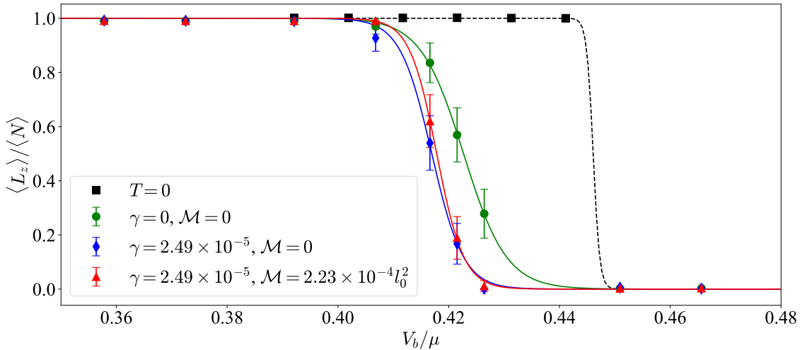
Figure 18: Final value of the average angular momentum per particle (which is equivalent to the final winding number) for the temperature T = 195\text{nK} and a barrier hold time of t_{\text{hold}} = 2.5\text{s} . There are several data-sets corresponding to T = 0 GPE simulations (black squares), and various subtheories of the SPGPE. Note that \mathcal{M} is given in units of l_0^2 , where l_0 = \sqrt{\hbar/m\omega_r} \approx 1.3\mu\text{m} is the radial lengthscale set by the trap. Each data set is fitted to a sigmoidal function: \langle L_z \rangle / \langle N \rangle = [\exp((V_b/\mu - \alpha)/\beta) + 1]^{-1} , where \alpha, \beta are the fitting parameters. Error bars give a 95% confidence interval in the data. Notably, the absence of energy-damping ( \gamma \neq 0, \mathcal{M} = 0 ) does not deviate significantly from the full SPGPE result ( \gamma \neq 0, \mathcal{M} \neq 0 ).
