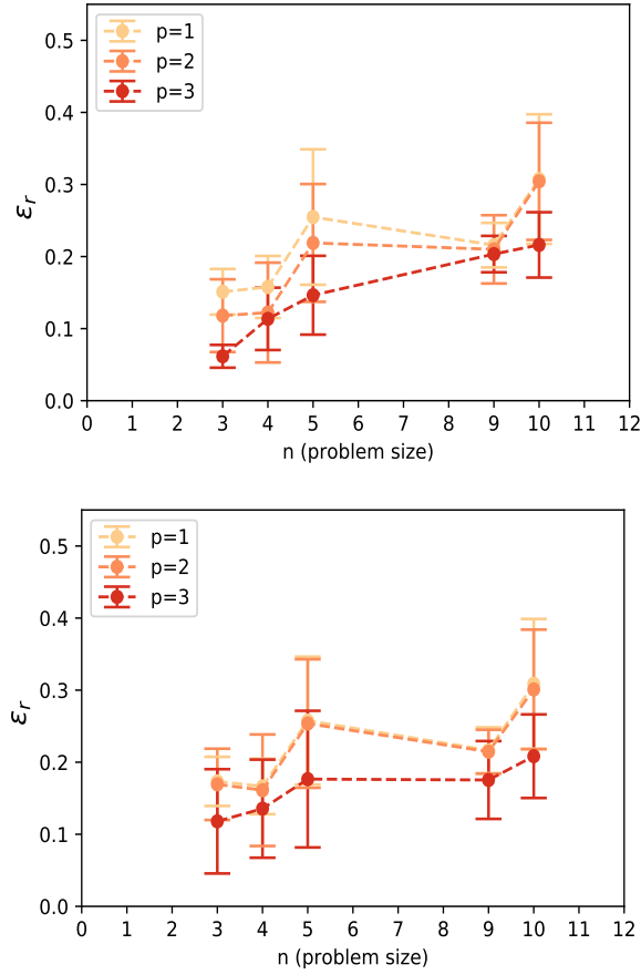
Figure 3: Comparison of converged final relative error (median), for p \in \{1, 2, 3\} , as a function of problem size n \in \{3, 4, 5, 9, 10\} , done on 5 problem instances per n with a budget of 200 iterations. (TOP) shows the results from the optimization having access to the exact waveform (statevector simulator), while (BOTTOM) shows the results using a shot-noise simulator with 2^{n+2} shots. For drawing the bottom plot, we use the best angles found using shot-based optimization and used the statevector QVM for one more run at those angles in order to compute the exact expectation value and corresponding relative error. These results are from the experiments described in Section 3.3.2.
