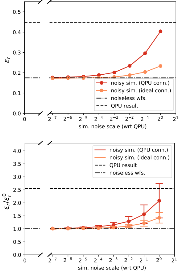
Figure 6: (TOP) Comparison of relative error \varepsilon_r with respect to the scaled noise model simulations for a typical 5 qubit problem instance (log scale). Noiseless waveform simulation as well as QPU results are also plotted for reference. (BOTTOM) Relative error factor \varepsilon_r/\varepsilon_r^0 with respect to the scaled noise model simulations (log scale). Here, \varepsilon_r^0 refers to the relative error observed in the case of the noiseless wavefunction simulator and \varepsilon_r/\varepsilon_r^0 measures \varepsilon_r as a factor of \varepsilon_r^0 . Values plotted on the y axis are medians (error bars are in Median Absolute Deviations) calculated from the values of the 30 selected 5 qubit problems. The QPU result in the bottom plot has a MAD of 1.04. Both plots are made with results from a QAOA depth of p = 1 , for device-limited coupling map restrictions (QPU conn.) and all-to-all connectivity (ideal conn.).
