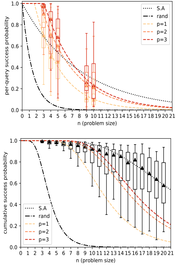
Figure 4: Comparison of success probabilities of sampling the ground state, for QAOA at depths p = 1, 2, 3 , Simulated Annealing and random sampling. (TOP) shows the success probability per-query and (BOTTOM) shows the cumulative success probability after 10 queries. The box plots indicate the nature of the experimental results (with medians as triangles) while curves in the figure are fitted to them. The QAOA results are from the statevector (no noise) experiments as described in Section 3.3.1 and the approach for comparing it with Simulated Annealing and random sampling is described in Section 3.4.4.
