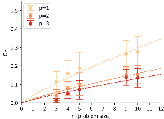
Figure 2: Comparison of converged final relative error \varepsilon_r (median), for p \in \{1, 2, 3\} , as a function of problem size n \in \{3, 4, 5, 9, 10\} . Simulations performed with access to the exact wave form (statevector QVM) done on 100 problem instances per n with an optimization budget of 200 iterations for p \in \{1, 2\} and 400 iterations for p = 3 . The dashed curves in the plot are fitted to the experimental data. The information presented in this figure is the output of experiments described in Section 3.3.1.
