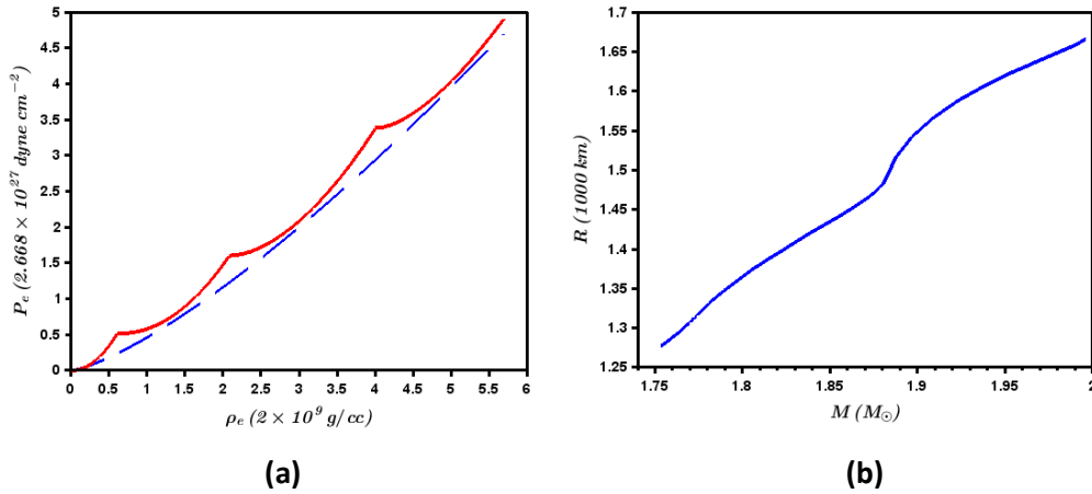
Figure 9: (a) EoS for constant magnetic field ( n = 0 ) of B_{cent} = 2 \times 10^{15} \text{ G} (red solid line) describing the central region of white dwarfs (see Eq. 51) and Chandrasekhar's EoS (dashed blue line) describing otherwise for \epsilon_{Fmax} = 18 , (b) corresponding mass–radius relation.
