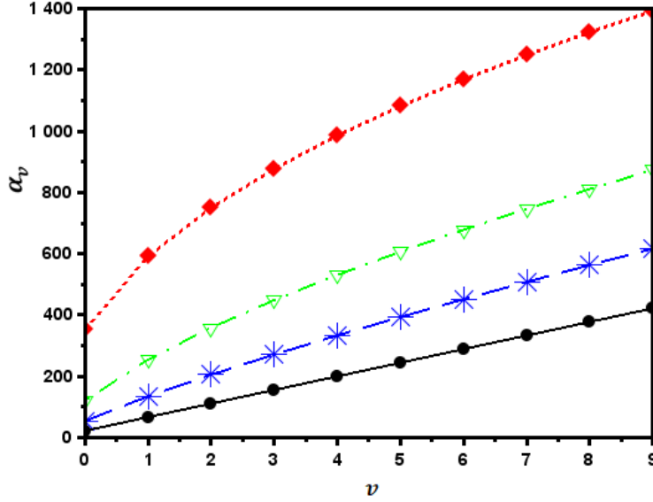
Figure 2: The variation of eigenvalue with eigen-index for B_0 = 10^{15} G pm ^{-n} , when n = 0 (black solid circles), -0.3 (blue dashed asterisks), -0.5 (green dot-dashed triangles) and -0.7 (red dotted diamonds). The lines represent the curves fitted with constants of Eq. (31).
