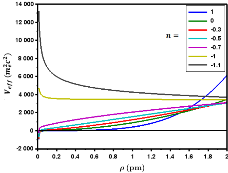
Figure 1: The variation of effective potential for different n for B_0 = 10^{15} G \text{pm}^{-n} . Here, the black horizontal line represents V_{eff} = 0 . Various potentials at \rho = 1 pm from bottom to top successively are for n = 1, 0, -0.3, -0.5, -0.7, -1, -1.1 .
