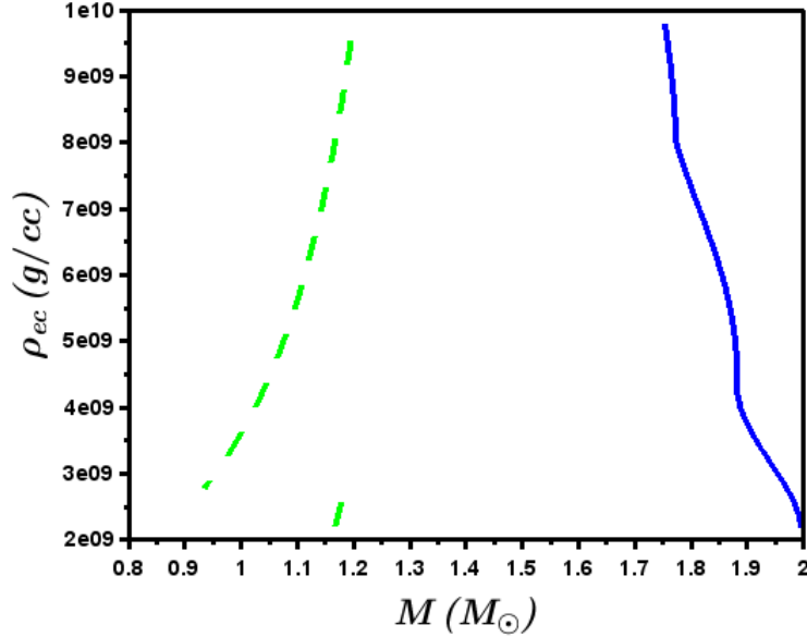
Figure 10: Comparison of M - \rho_{ec} relation (solid blue line) with that of the hypothetical case with Chandrasekhar's EoS but Lorentz force intact (dashed green line).
