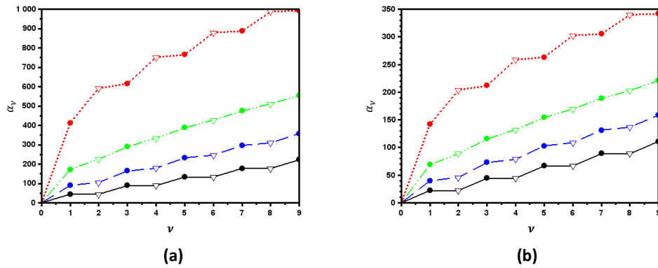
Figure 3: The variation of eigenvalue with the eigen-index for n = 0 (black solid line), -0.3 (blue dashed line), -0.5 (green dot-dashed line) and -0.7 (red dotted line) for (a) B_0 = 10^{15} G pm ^{-n} , and (b) B_0 = 5 \times 10^{14} G pm ^{-n} , and m = 0 . Here the levels for -\sigma \cdot \mathbf{B} ( -B_0 ) and +\sigma \cdot \mathbf{B} ( +B_0 ) are marked by the solid circles and triangles respectively.
