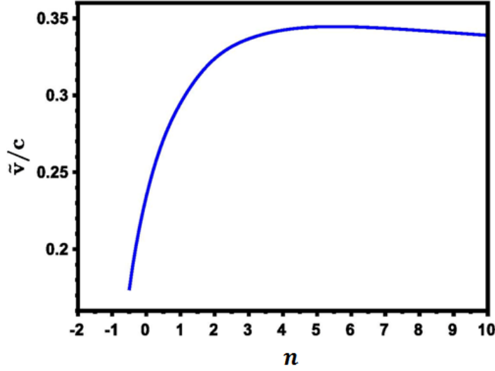
Figure 11: Variation of quantum speed of spin-up electron for transition from ground state to first excited state with different n at B_0 = 10^{16} G pm ^{-n} .
