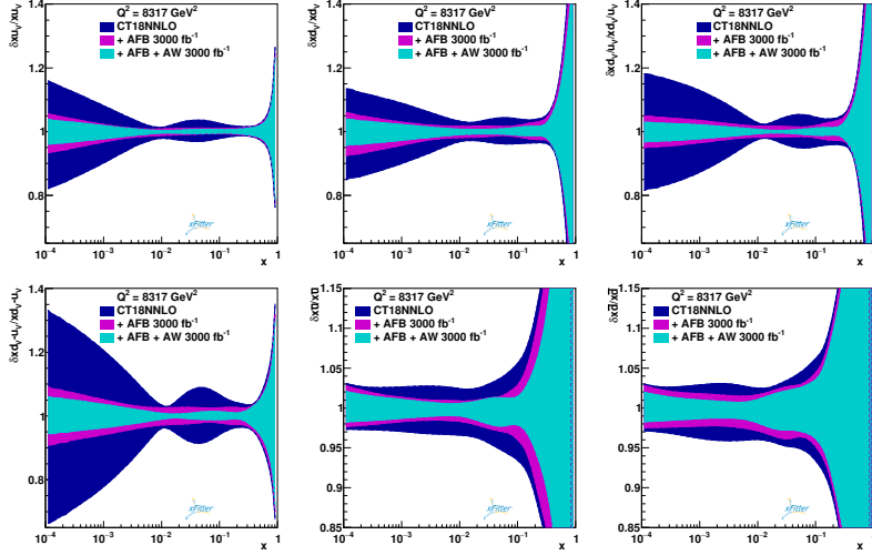
Figure 2: Same as in Fig. 1 but for an integrated luminosity of 3000 \text{ fb}^{-1} .
