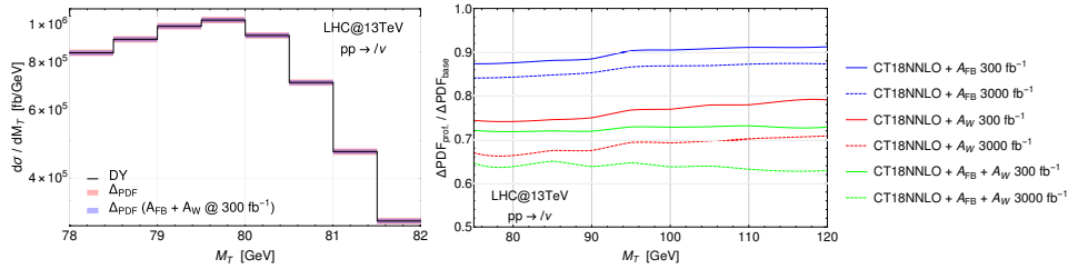
Figure 3: (left) Charged-current DY transverse mass distribution with PDF error; (right) relative improvement of PDF error on the transverse mass spectrum due to profiling based on A_{FB} , A_W and their combination.
