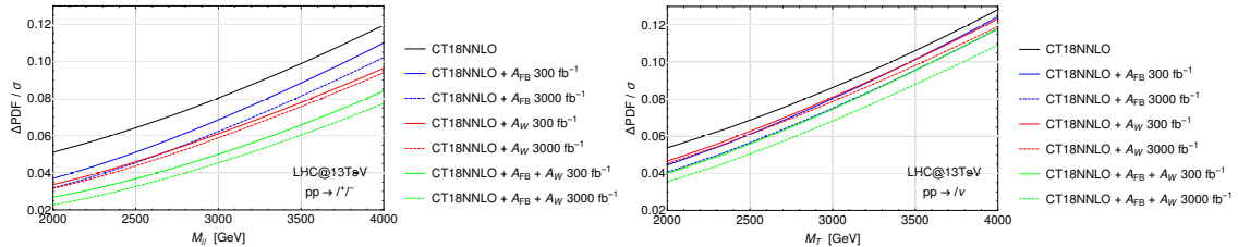
Figure 4: Relative PDF error on the invariant mass spectrum of the neutral DY channel (left) and on the transverse mass spectrum of the charged DY channel (right).
