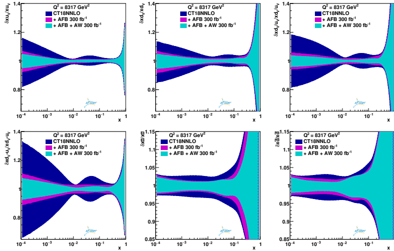
Figure 1: Original CT18NNLO [13] (blue) and profiled distributions of selected PDFs using either A_{FB} (pink) or both A_{FB} and A_W (cyan) pseudodata corresponding to an integrated luminosity of 300 \text{fb}^{-1} .
