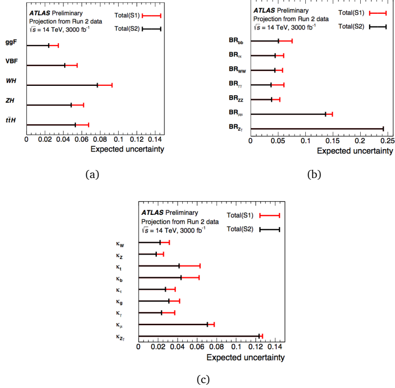
Figure 2: Expected uncertainty on the measurements of the cross sections for the ggF , VBF , WH , ZH and ttH production modes normalised to their SM predictions assuming SM branching fractions (a), the expected uncertainty on the branching ratio measurements for the \gamma\gamma , ZZ , WW , \tau\tau , bb , \mu\mu (b) and Z\gamma decay channels normalised to their SM predictions assuming SM production cross section and the expected uncertainty on the measurement of each Higgs boson coupling modifier per particle type with effective photon, gluon and Z\gamma couplings (c), for the two systematic uncertainties scenarios S1 (red) and S2 (black) [23].
