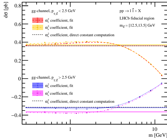
Figure 2: The same as the lower panel of Fig. 1, focussing on the gg -channel in two p_{T, \ell\bar{\ell}} regions. The result of a numerical fit to the difference between the massive and logarithmic cross-sections is shown, and compared to the direct calculation of the zero mass constant at \mathcal{O}(\alpha_s^2) .
