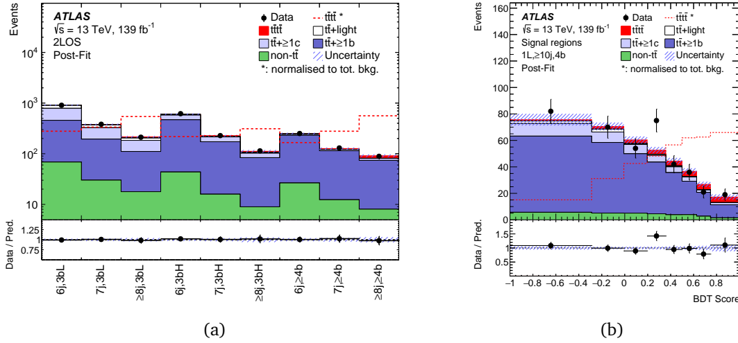
Figure 1: Post-fit agreement between t\bar{t}t\bar{t} data and simulation in various regions: (a) Yields for each SR and CR in 2LOS channel; (b) BDT distribution in (1L,10j,4b) SR. Shaded bands represent both statistical and systematic uncertainties [7].
