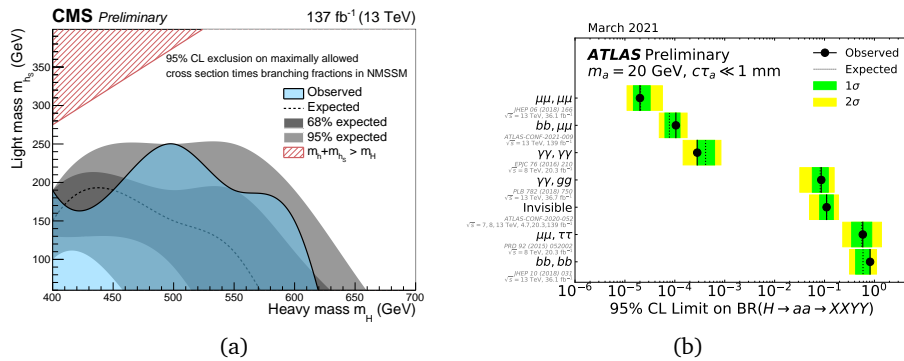
Figure 2: Measured 95% confidence level exclusion limits of searches for BSM physics. Left: Exclusion limits for the production of new Higgs bosons H and h_S as a function of their respective mass in H \rightarrow h_S h \rightarrow \tau\tau bb events interpreted within the NMSSM model (CMS [27]). Right: Summary of upper limits on SM Higgs boson decays to new light scalars in various decay channels (ATLAS [32]).
