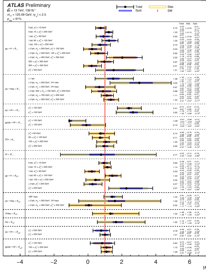
Figure 1: The ATLAS collaboration’s STXS measurements of ggF , VBF , VH and ttH production in the H \rightarrow \gamma\gamma and H \rightarrow ZZ^* channel and VH production in the H \rightarrow bb channel that enter in the statistical combination [15].
