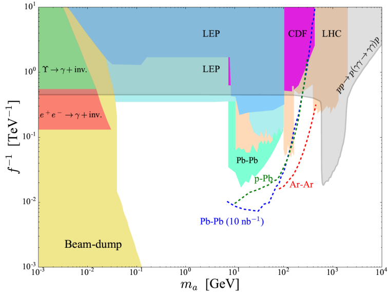
Figure 6: Coupling vs ALP mass sensitivity plot. The reach using the measurement of two intact protons and the two photons for photon-induced processes is shown as a grey area.
