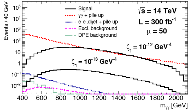
Figure 4: Number of events as a function of the diphoton mass for signal and background for exclusive \gamma\gamma production.
