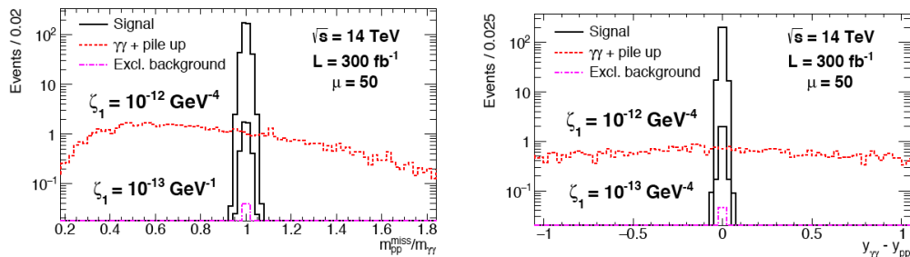
Figure 5: Mass ratio and rapidity difference between the pp and \gamma\gamma information for signal (in full line) and pile up background (dashed line).
