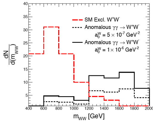
Figure 7: WW mass distribution for exclusive WW production (SM is red dashed line and anomalous couplings in full ball line).
