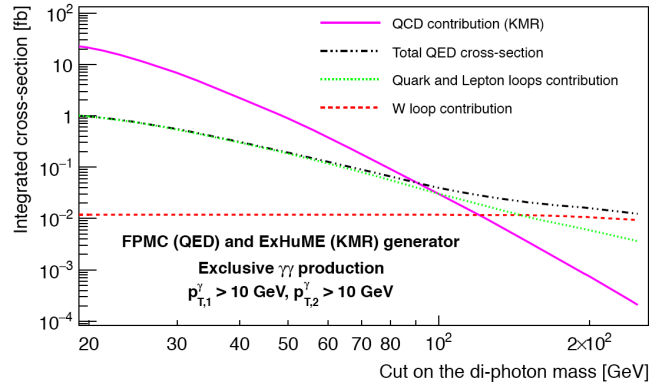
Figure 3: Cross section of exclusive diphoton production above a given diphoton mass given in abscissa for QCD (full line) and QED (dashed dotted line) processes.
