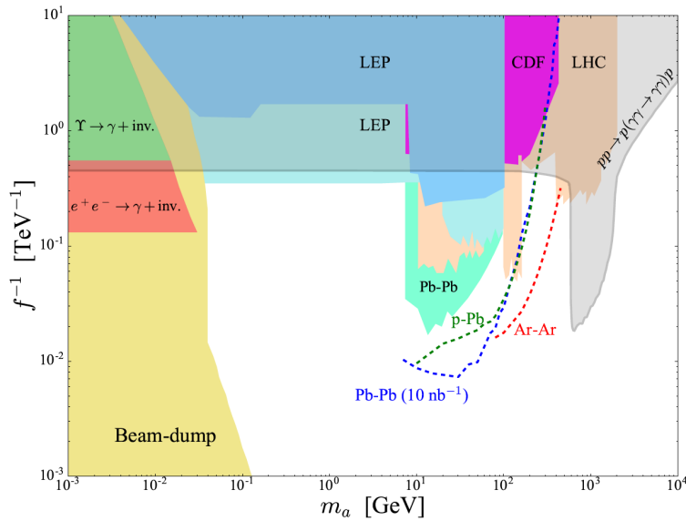
Figure 6: Coupling vs ALP mass sensitivity plot. The reach using the measurement of two intact protons and the two photons for photon-induced processes is shown as a grey area.
