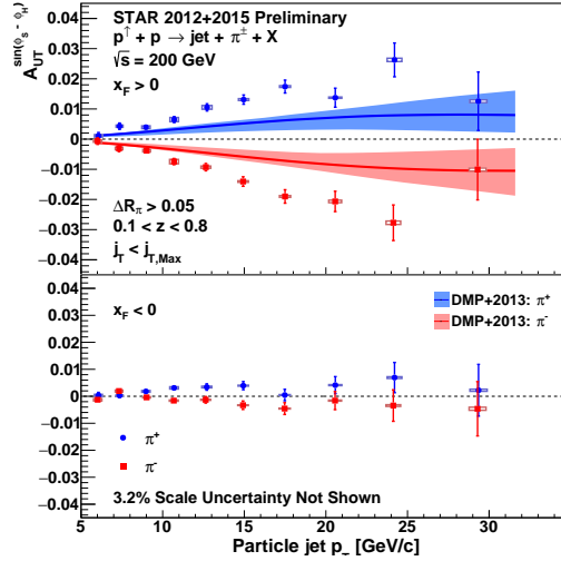
Figure 2: STAR Collins asymmetry: A_{UT}^{sin(\phi_s-\phi_H)} as a function of the particle-jet p_T in forward ( x_f > 0 ) (top panel) and backward ( x_f < 0 ) jet scattering directions (bottom panel), for the \pi^\pm within jets, compared with the theoretical calculation from [15].
