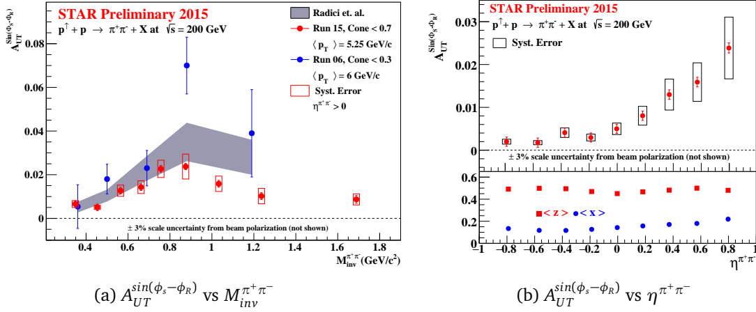
Figure 1: STAR IFF asymmetries: 1a) A_{UT}^{sin(\phi_s-\phi_R)} as a function of invariant mass of two oppositely-charged pions, M_{inv}^{\pi^+\pi^-} , in \eta^{\pi^+\pi^-} > 0 region, compared with the theoretical calculation from [13]. The cone cut ( \sqrt{(\eta^{\pi^+} - \eta^{\pi^-})^2 + (\phi^{\pi^+} - \phi^{\pi^-})^2} < 0.7 ) ensures that the \pi^+ and \pi^- are close enough in \eta - \phi space. 1b) A_{UT}^{sin(\phi_s-\phi_R)} as a function of \eta^{\pi^+\pi^-} , integrated over M_{inv}^{\pi^+\pi^-} and p_T^{\pi^+\pi^-} (top panel). The quark ( z ) and ( x ), in the corresponding \eta^{\pi^+\pi^-} bins, are shown in the bottom panel.
