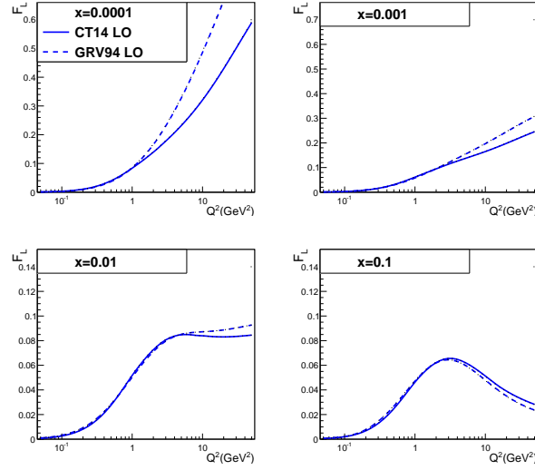
Figure 1: The results from the model for F_L for two different PDFs, CTEQ14LO and GRV94LO as a function of Q^2 for fixed values of x .
