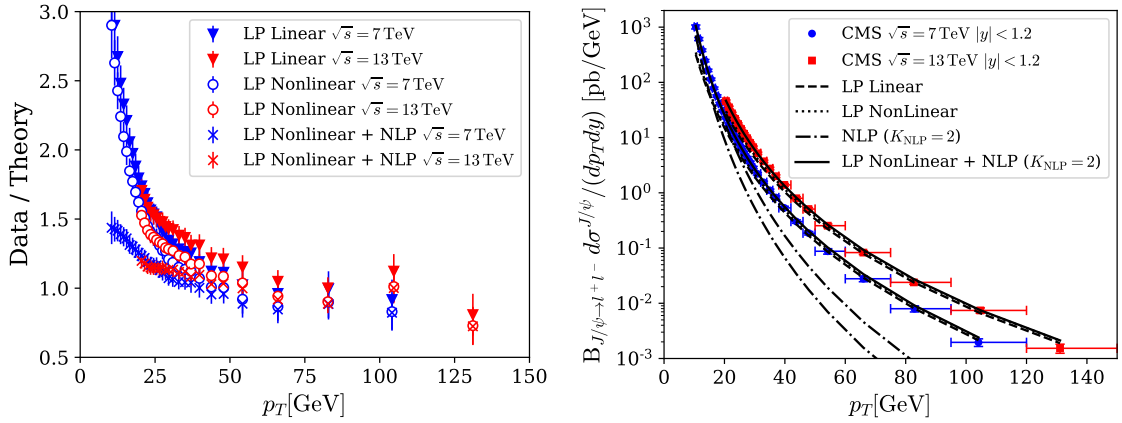
Figure 3: (Left): Ratios of CMS data to theoretical calculations for hadronic J/\psi production at the LHC. (Right): Prompt J/\psi production in p + p collisions at mid-rapidity at the LHC with K_{\text{NLP}} = 2 and (\alpha, \beta) given in the text.
