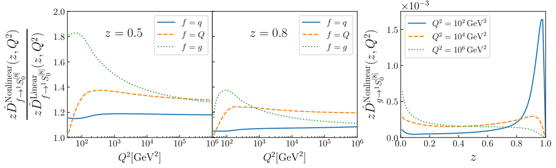
Figure 2: (Left): Ratios of the LP FFs with the nonlinear corrections to that without the nonlinear corrections for \hat{D}_{f \rightarrow 1S_0^{[8]}} \equiv D_{f \rightarrow H} / \langle \mathcal{O}_{1S_0^{[8]}}^H \rangle . (Right): The \hat{D}_{g \rightarrow 1S_0^{[8]}} LP FF with the nonlinear corrections as a function of z .
