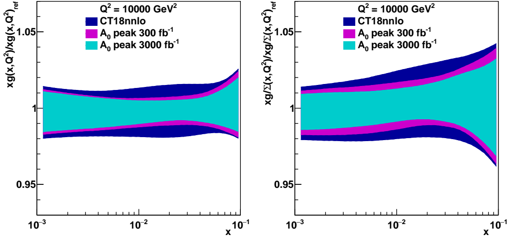
Figure 1: The gluon ( xg ) and gluon/Sea ( xg/\Sigma ) PDFs in the original CT18NNLO analysis (blue) and profiled using A_0 pseudodata corresponding to integrated luminosities of 300 fb -1 (magenta) and 3 ab -1 (cyan) in the region 80 GeV < M < 100 GeV and |Y| < 3.5 .
