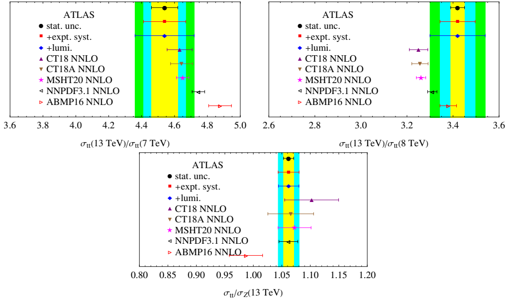
Figure 4: Top-antitop production cross section ratios for \sqrt{s} = 13, 7, 8 TeV and the ratio \sigma_{t\bar{t}}/\sigma_Z at 13 TeV, compared with the ATLAS measurements [22].
