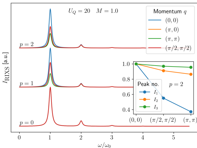
FIG. 4. The RIXS spectrum obtained using the MA method for different \mathbf{q} momentum transfers, for increasing cluster sizes p = \{0, 1, 2\} . Parameters are t = 5, U_Q = 20, M = 1, \Gamma = 2, \eta = 0.05 .
