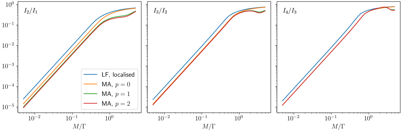
FIG. 7. The first three phonon peak ratios as a function of coupling M/\Gamma . The linear dependence implies RIXS might be a good technique for directly determining the e - p coupling. Parameters for the O K -edge: t = 5, U_Q = 20, \Gamma = 2 .
