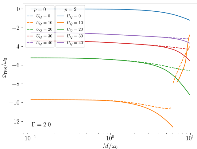
FIG. 3. Resonance position as determined from the maximum of the XAS spectrum, Eq. (21), as a function of e - p coupling M and for a wide range of core hole potential values U_Q ; t = 5, \Gamma = 2 . The difference between the p = 0 (dashed lines) and p = 2 (solid lines) solutions is visible at strong coupling M > 1 . The discontinuity at U_Q = 10 is due to bimodality of the XAS spectrum in this regime.
