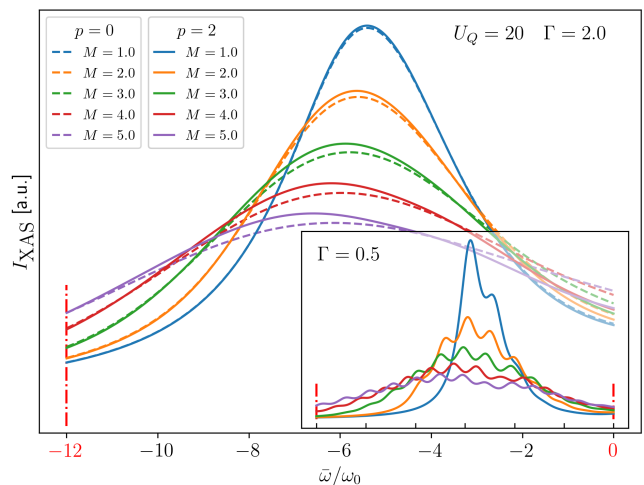
FIG. 2. A comparison of the XAS spectra, as obtained using the MA method for p = 0 (dashed lines) and p = 2 (solid lines). Results are shown in the main panel for parameters t = 5 , U_Q = 20 , and \Gamma = 2 . The inset shows results obtained from a p = 2 calculation for the same parameter set but with \Gamma = 0.5 . Note that the x-axis of the inset spans the same range as the main panel.
