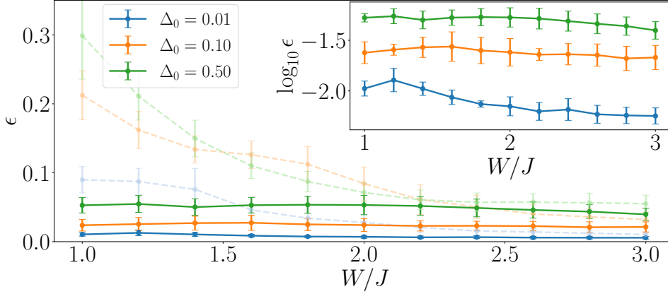
Figure 8: Median relative error \epsilon in the many-body eigenenergies obtained from the flow equation method for L = 12 and three different microscopic interaction strengths \Delta_0 , using \phi = (1 + \sqrt{5})/2 (the golden ratio) and averaged over N_s = 2048 random values of the phase \theta , computed with respect to the results obtained from exact diagonalization. The error bars represent the median average deviation over different random values of the phase \theta . The dashed lines represent the result of the older implementation used in Refs [41,42]: as this is much larger than the error in the newer method, we show in the inset the results for the newer method only, on a log scale. We see that the relative error is roughly flat with respect to disorder, but rises as the interaction strength increases. We therefore conclude that the truncation in the running Hamiltonian (Eq. 15) is the main source of error in this procedure, as expected, but that crucially there is no runaway error in the delocalized phase as seen in the older flow equation implementation (dashed lines).
