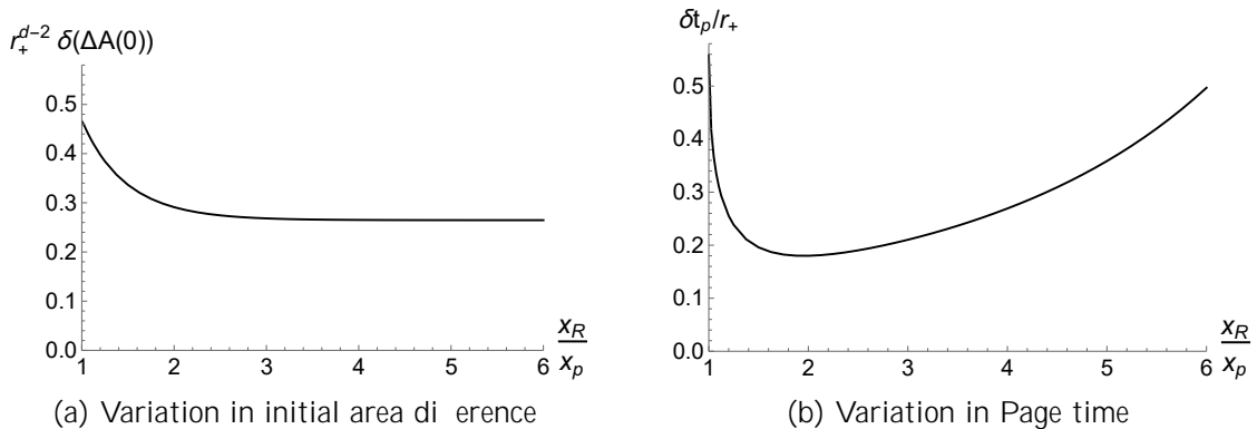
Figure 11: The variations in the (a) initial area difference and the (b) Page time as functions of the radiation region. We compute these quantities up to x_R/x_p = 6 , at which point our numerics become too noisy to be taken as reliable. Nonetheless, even within this range the numerics indicate that the variation in initial area difference monotonically falls while the variation in the Page time drops then rises.
