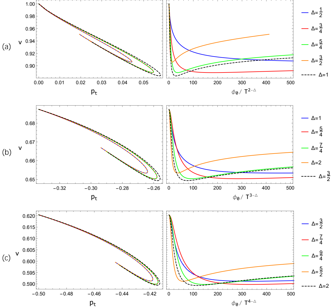
Figure 8: Entanglement velocity v as a function of p_t and \phi_0/T^d for (a) d = 2 , (b) d = 3 , and (c) d = 4 . Each plot starts at its AdS-Schwarzschild value from (3.39). The p_t curves obey a \Delta \pm d - \Delta symmetry—they are sensitive to m^2 .
