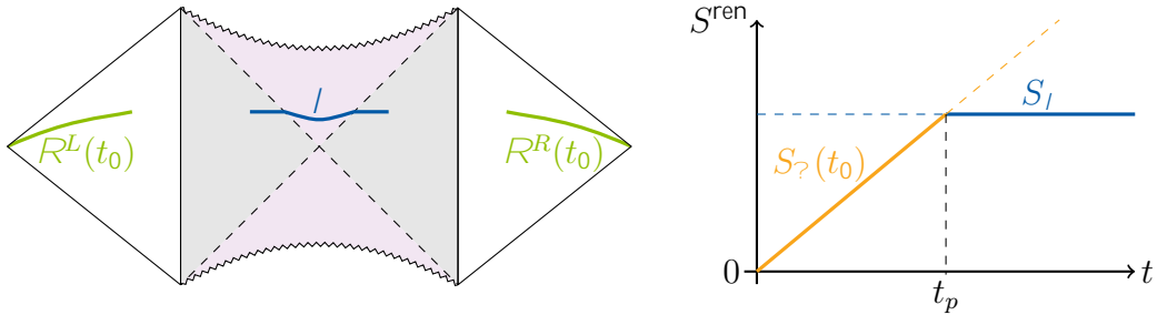
Figure 2: On the left is the two-sided thermal configuration of (II) featuring both the t = t_0 radiation region R^L(t_0) [ R^R(t_0) and the island I which emerges at late times. The right figure is a sketch of the (eternal) Page curve depicting (renormalized) entanglement entropy versus time—initially the time-dependent no-island entropy S_? is minimal, but it eventually exceeds the non-trivial island entropy S_I . This curve can be obtained by computing (renormalized) areas in the (III) configuration.
