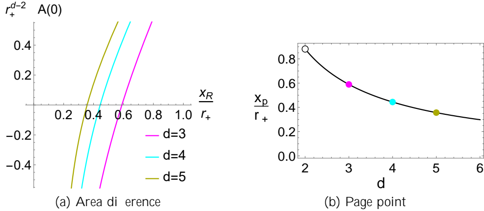
Figure 6: (a) The area difference \Delta A(0) (3.23) versus x_R (3.19) for d = 3, 4, 5 and (b) the Page point x_p as a function of (analytically-continued) d > 2 , all in the AdS-Schwarzschild geometry and in r_+ units. The area difference in each dimension monotonically increases with x_R , crossing 0 at a particular value beyond which we have Page curves. The Page point thus approaches the brane as we increase d .
