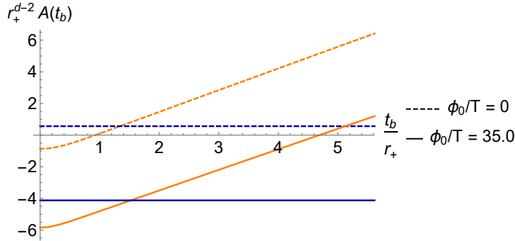
Figure 9: The Page curves for \phi_0/T = 0 and \phi_0/T = 35.0 with d = 3 , \Delta = 2 , presented in terms of the area A and boundary time t_b in units of r_+ . The orange curves are Hartman-Maldacena surface areas while the blue curves are island surface areas. For both, we observe a phase transition from the former to the latter at finite boundary times—the respective Page times given these deformations.
