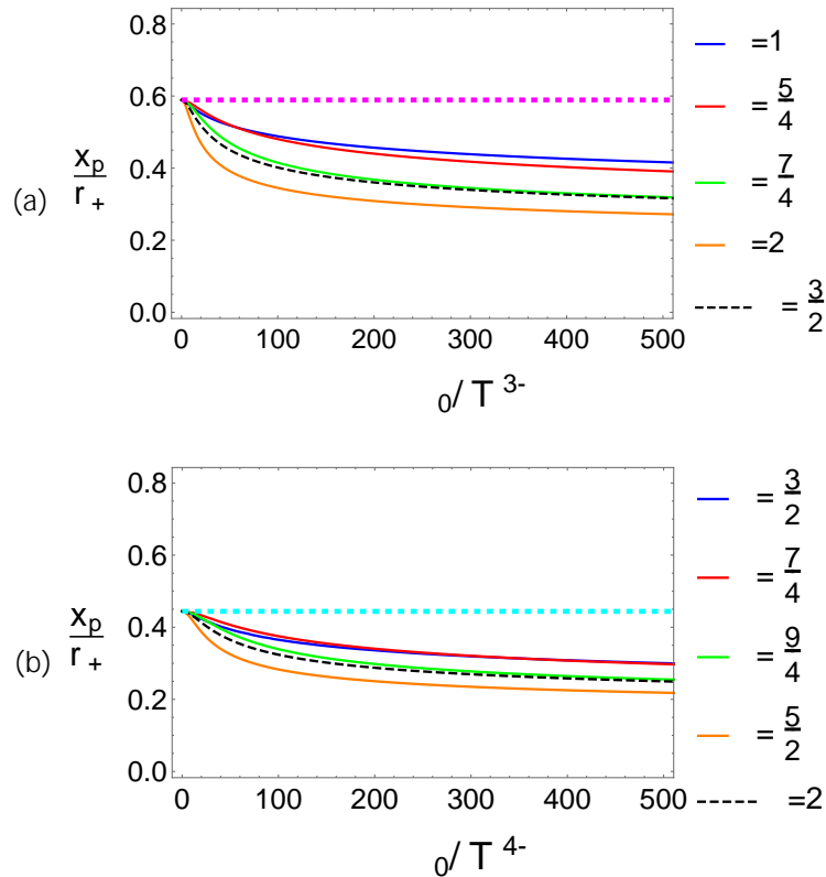
Figure 7: The Page point x_p as a function of \phi_0/T^d for (a) d = 3 and (b) d = 4 (the cases in Section 3.2). The horizontal lines are at the AdS-Schwarzschild Page points shown in Figure 6. The Page point decreases as \phi_0/T^d increases.
