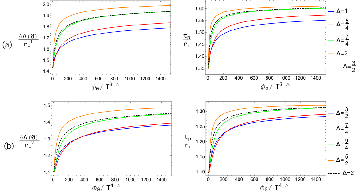
Figure 10: The initial area difference \Delta A(0) and the Page time t_p plotted as functions of \phi_0/T^d for (a) d = 3 and (b) d = 4 , all for various \Delta . The axes are in r_+ units.
