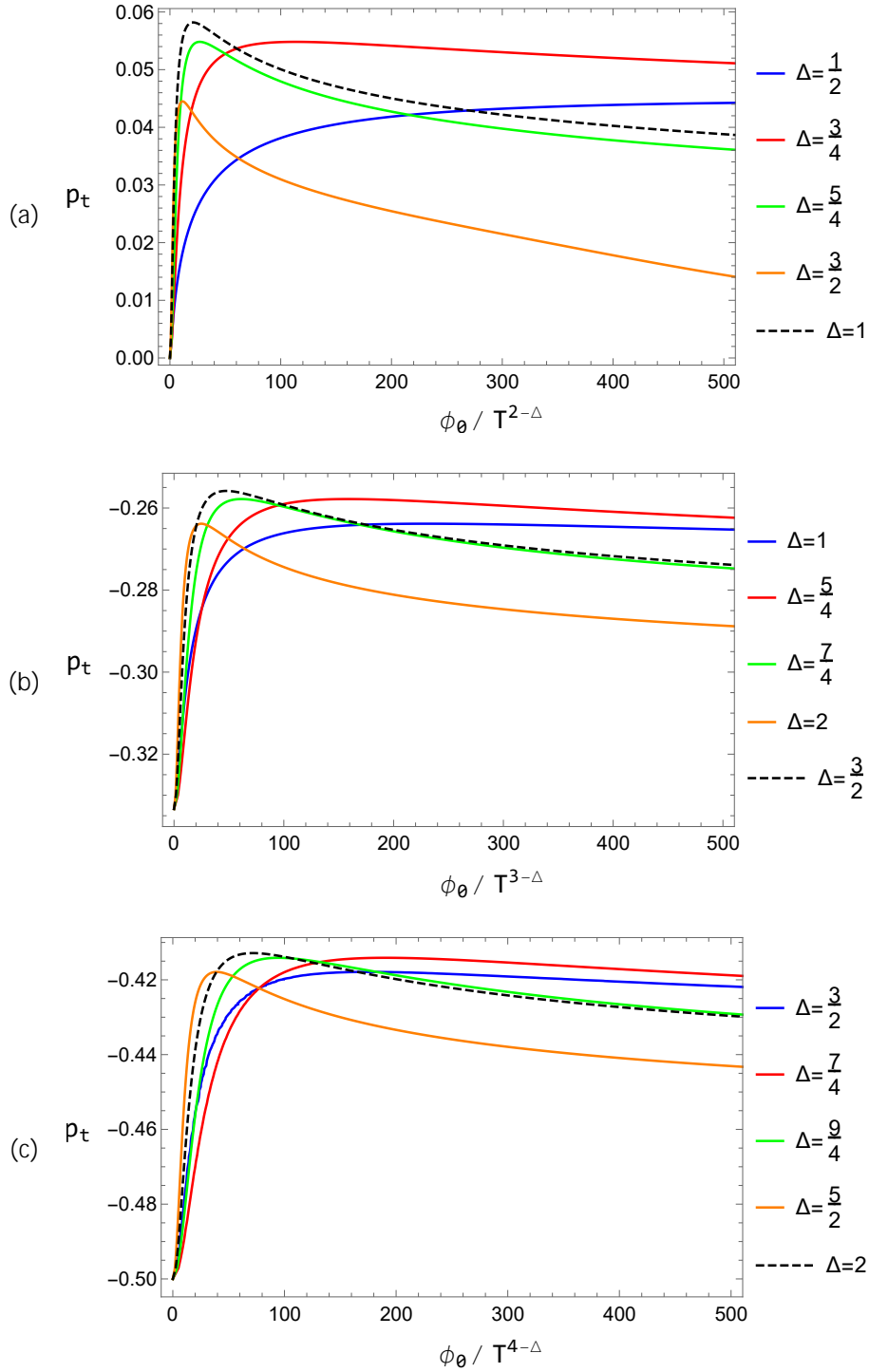
Figure 3: The emergent Kasner exponent p_t versus the dimensionless deformation parameter \phi_0/T^d for various d and \Delta , computed via a numerical shooting method outlined in Appendix B. We show the results for (a) d = 2 , (b) d = 3 , and (c) d = 4 . The dashed lines correspond to \Delta = d/2 .
