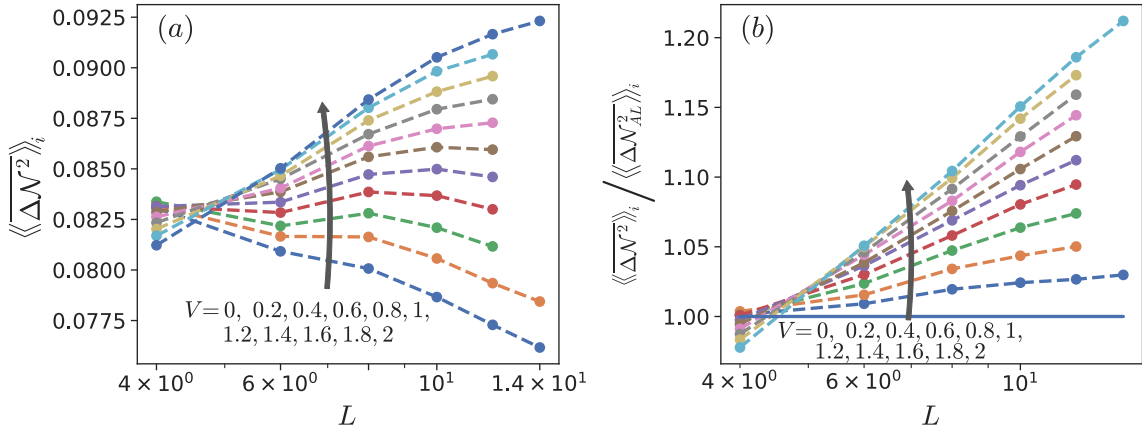
Figure 8: (a) Time-averaged particle fluctuations \langle\langle \Delta N^2 \rangle\rangle_i in dependence of system size L averaged over all possible initial states. (b) Same as in (a) but relative to the fluctuations in the non-interacting case \langle\langle \Delta N_{AL}^2 \rangle\rangle_i . The data are averaged over 10000 disorder realizations.
