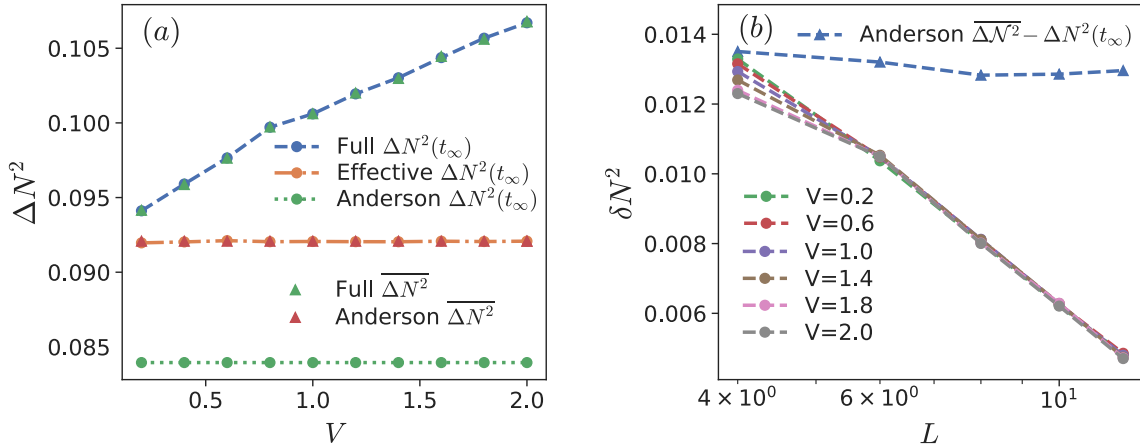
Figure 10: (a) Comparison of the time-averaged fluctuations \overline{\Delta N^2} obtained from Eq. (15) where the assumption (14) has been used (triangles) with \Delta N^2(t \rightarrow \infty) (dots) where the assumption (14) has not been used for the full microscopic model, the effective model, and the Anderson model for L = 12 . (b) \delta N^2 , Eq. (17), for the microscopic model and different interaction strengths. In all cases, the data are consistent with \delta N^2 \sim \exp(-L) . For comparison, the Anderson case is shown as well. For L \leq 10 the data is averaged over 50000 disorder realizations, and 20000 for L = 12 .
