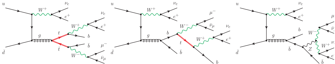
Figure 3: Representative Feynman diagrams for the double, single and non-resonant contributions to the pp \rightarrow e^+ \nu_e \mu^- \nu_\mu e^+ \nu_e b \bar{b} amplitude. Figure taken from Ref. [7].
