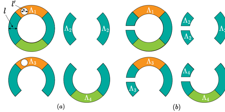
Figure 7: Pictorial representation of l -genuine topological difference. The typical size of the sketched domain is l . (a) A l' patch has been applied to the sets of domains E_{\Lambda_1\Lambda_2} and since l' < l the sets shows the same genuine topological difference, indeed n_{\partial}(E_{\Lambda_1\Lambda_2}) = 3 + 2 , n_{\partial}(E_{\Lambda_3\Lambda_4}) = 2 + 1 and n_{\partial}(E_{\Lambda_1\Lambda_2}) - n_{\partial}(E_{\Lambda_3\Lambda_4}) = 2 , cfr. Fig. 6. (b) the sets are patched with a patch whose size is l' \geq l which change the genuine topological difference, indeed n_{\partial}(E_{\Lambda_1\Lambda_2}) = 1 + 3 , n_{\partial}(E_{\Lambda_3\Lambda_4}) = 2 + 2 and n_{\partial}(E_{\Lambda_1\Lambda_2}) - n_{\partial}(E_{\Lambda_3\Lambda_4}) = 0 \neq 2 .
