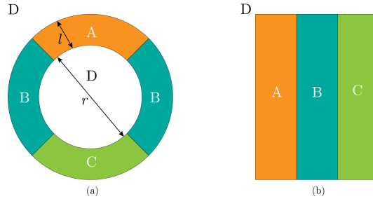
Figure 2: (a) The graph configuration to define the topological entropy, i.e. I(A; C|B) . l is the feature size of this graph configuration and l \sim O(N^2) , where N^2 is the whole lattice size, while r is radius of this topologically non trivial domain. (b) I(A; C|B) = 0 in this simple graph configuration, even though there is long-range entanglement of the ground state.
