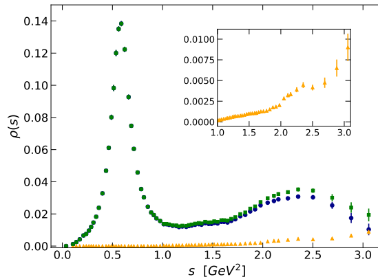
Figure 2: Total vector isovector spectral function (green) obtained from the addition of the dominant modes (blue) and the residual modes (yellow). (Figure extracted from Ref. [3].)
