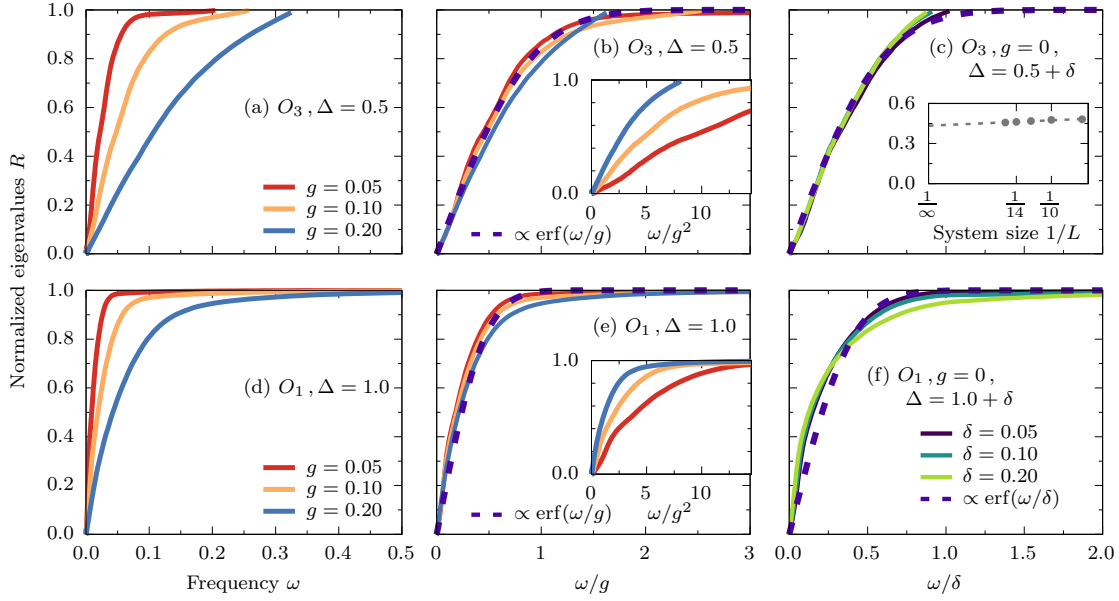
Figure 6: Cumulative spectral functions R_\alpha(\omega) , Eq. (14), as calculated for L = 16 system. We show results for (a) O_3 with \Delta = 1/2 and (d) for O_1 with \Delta = 1 . Panels (b) and (e) show respectively the same data but with rescaled frequency \omega/g (main panels) and \omega/g^2 (insets). Panels (c) and (f) show results for integrable system ( g = 0 ) but for shifted anisotropy parameters \Delta = 0.5 + \delta and \Delta = 1 + \delta , respectively. Dashed curves show fittings with the error function. Inset in (c) shows finite-size scaling of the stiffness C_3(t \rightarrow \infty) for \Delta = 0.5 and g = 0 .
