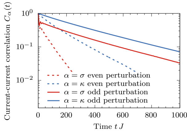
Figure 5: Current correlation function C_\alpha(t) for the perturbation, Eq. (10), breaking the parity symmetry P , as compared with P -preserving perturbation Eq. (1). Calculated for L = 28 , \Delta = 0.5 , g = 0.15 , and S_{\text{tot}}^z = 0 .
