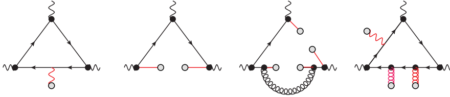
Figure 3: Topologies giving the different contributions to the studied OPE.
