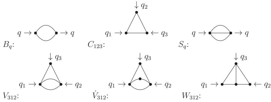
Figure 4: Master integrals entering into the two-loop calculation after applying scalar reduction. Figure reused from [5].
