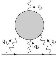
Figure 1: HLbL contribution to g-2 . Figure reused from [5].
