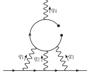
Figure 2: Quark condensate contribution to HLbL. In the static q_4 \rightarrow 0 limit the quark propagator on the left diverges. Figure reused from [3].
