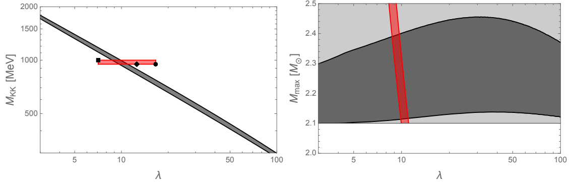
Figure 4: Left panel: Allowed range according to the astrophysical constraints in the \lambda - M_{\text{KK}} plane (doubly logarithmic), obtained by applying the construction of Fig. 3 for each \lambda . The three symbols mark the parameter pairs from the QCD fits of table 1, and we use them to define a "QCD window" (red). Right panel: Constraints for the maximal mass of the neutron star as a function of the 't Hooft coupling \lambda . The light gray band gives the constraint from astrophysical data. The dark gray band and the red band arise from applying the constraints of the left panel.
