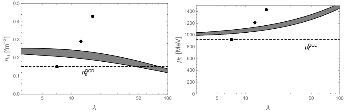
Figure 5: Saturation density of symmetric nuclear matter (left) and corresponding onset chemical potential (right) as functions of \lambda for the astrophysically allowed parameter band, see left panel of Fig. 4, and for the three fits of table 1. The dashed horizontal lines indicate the real-world values.
