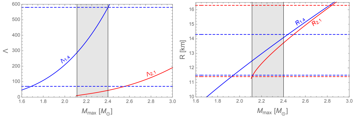
Figure 3: Tidal deformability \Lambda and radius R for a 1.4-solar-mass star (blue solid) and a 2.1-solar-mass star (red solid) as a function of the maximal mass M_{\max} . Here we have fixed the 't Hooft coupling \lambda = 10 and the surface tension \Sigma = 1 \text{ MeV}/\text{fm}^2 , and different values of M_{\max} are obtained by varying the second model parameter M_{\text{KK}} . The horizontal dashed lines indicate the astrophysical constraints for \Lambda_{1.4} , R_{1.4} , and R_{2.1} . Beyond the shaded region at least one of the constraints is violated. As a consequence, for this particular value of the 't Hooft coupling, we obtain 2.11 M_{\odot} \lesssim M_{\max} \lesssim 2.40 M_{\odot} and new bounds for \Lambda_{1.4} , R_{1.4} , \Lambda_{2.1} , R_{2.1} , for instance 288 \lesssim \Lambda_{1.4} \lesssim 580 .
