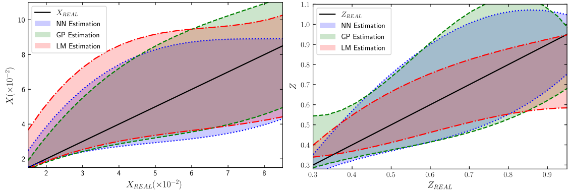
Figure 18: Correlation plots for X = x_1 (left) and X = z (right). We defined the error bands following the strategy mentioned in App. A, and present the results for the neural network (NN, blue), Gaussian process (GP, green) and the linear method (LM, red) estimations.
