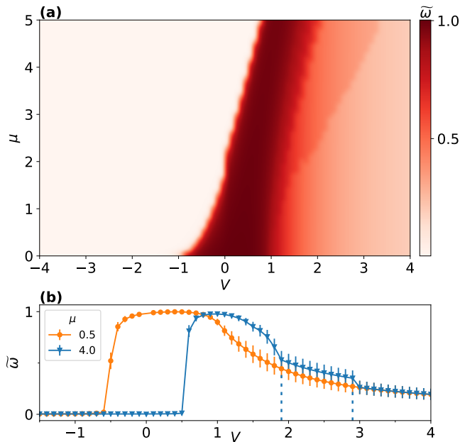
FIG. 7. Convolutional neural networks. (a) Predictions \tilde{\omega} of the phase diagram of the interacting Hamiltonian carried out by means of the CNN ensemble. The topological phase is correctly predicted (dark red region). (b) Two cuts of the phase diagram showing the predictions \tilde{\omega} and their relative standard errors as a function of V for different \mu . For the points with \mu \gtrsim 1 in the CDW phase it is possible to see the appearance of discontinuities (indicated by dashed vertical lines) for the values \tilde{\omega} that correspond to the onset of the incommensurate CDW phase.
