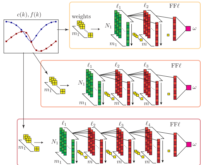
FIG. 6. Structure of the CNNs forming the ensemble. The input for the CNNs is a 2 \times L dataset with the correlation functions c(k), f(k) . First, the input is filtered by a layer of m_1 2D convolutional weights (in yellow) trained independently on each network. Each weight produces one array of length N_1 = L - 1 (the first set of green columns denoted by \ell_1 ) for a total of m_1 arrays. Then each network has a different number of additional hidden layers (columns in red): \ell_2, \ell_3, \ell_4 from the top. Each of these layers performs a 1D convolution using the weights in yellow. The last convolution always has one single weight in order to produce a single array. The last layer is a feed-forward layer (FFl) with one final output neuron that gives a real number which is the predicted winding number \omega by the network. All the resulting winding numbers from the different CNNs that constitute the ensemble are then averaged to give the predicted winding number \tilde{\omega} (Eq. (11)).
