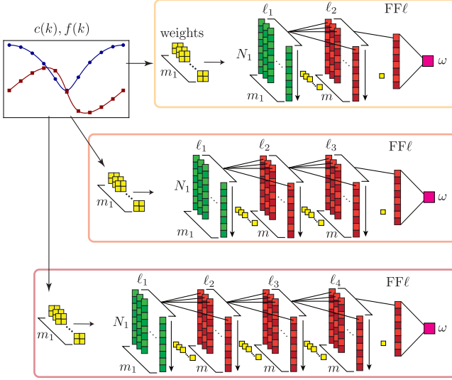
FIG. 7. Structure of the CNNs forming the ensemble. The input for the CNNs is a 2 \times L dataset with the correlation functions c(k), f(k) . First, the input is filtered by a layer of m_1 2D convolutional weights (in yellow) trained independently on each network. Each weight produces one array of length N_1 = L - 1 (the first set of green columns denoted by \ell_1 ) for a total of m_1 arrays. Then each network has a different number of additional hidden layers (columns in red): \ell_2, \ell_3, \ell_4 from the top. Each of these layers performs a 1D convolution using the weights in yellow. The last convolution always has one single weight in order to produce a single array. The last layer is a feed-forward layer (FFl) with one final output neuron that gives a real number which is the predicted topological indicator \omega by the network. All the resulting topological indicators from the different CNNs that constitute the ensemble are then averaged to give the predicted topological indicator \tilde{\omega} (Eq. (11)).
