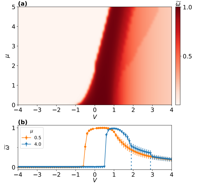
FIG. 8. Convolutional neural networks. (a) Predictions \tilde{\omega} of the phase diagram of the interacting Hamiltonian carried out by means of the CNN ensemble. The topological phase is correctly predicted (dark red region). (b) Two cuts of the phase diagram showing the predictions \tilde{\omega} and their relative standard errors as a function of V for different \mu . For the points with \mu \gtrsim 1 in the CDW phase it is possible to see the appearance of discontinuities (indicated by dashed vertical lines) for the values \tilde{\omega} that correspond to the onset of the incommensurate CDW phase.
