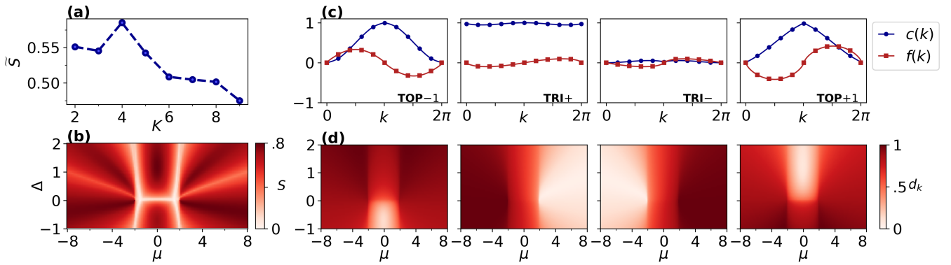
FIG. 4. Non-interacting Hamiltonian: k-means clustering. (a) Values of the silhouette score \tilde{S} as a function of the number of clusters K . The maximum value is reached at K = 4 and suggests the best number of centroids for the dataset points. (b) Reconstructed phase diagram of the non-interacting model (with K = 4 centroids) through the average silhouette S of every data point. The critical lines are clearly visible because the correlation functions of critical points have similar distances between two centroids. (c) Centroids obtained by applying k-means algorithm with K = 4 . Every centroid resembles the correlation functions of the four different regions: topological with \nu = -1 , the two trivial phases with \nu = 0 and topological with \nu = +1 , from left to right. (d) Distances d_k of the correlation functions for each point of the phase diagram from the corresponding k -th centroid (plotted in the corresponding panel above). The points belonging to the same phase show minimal distance to the same centroid.
