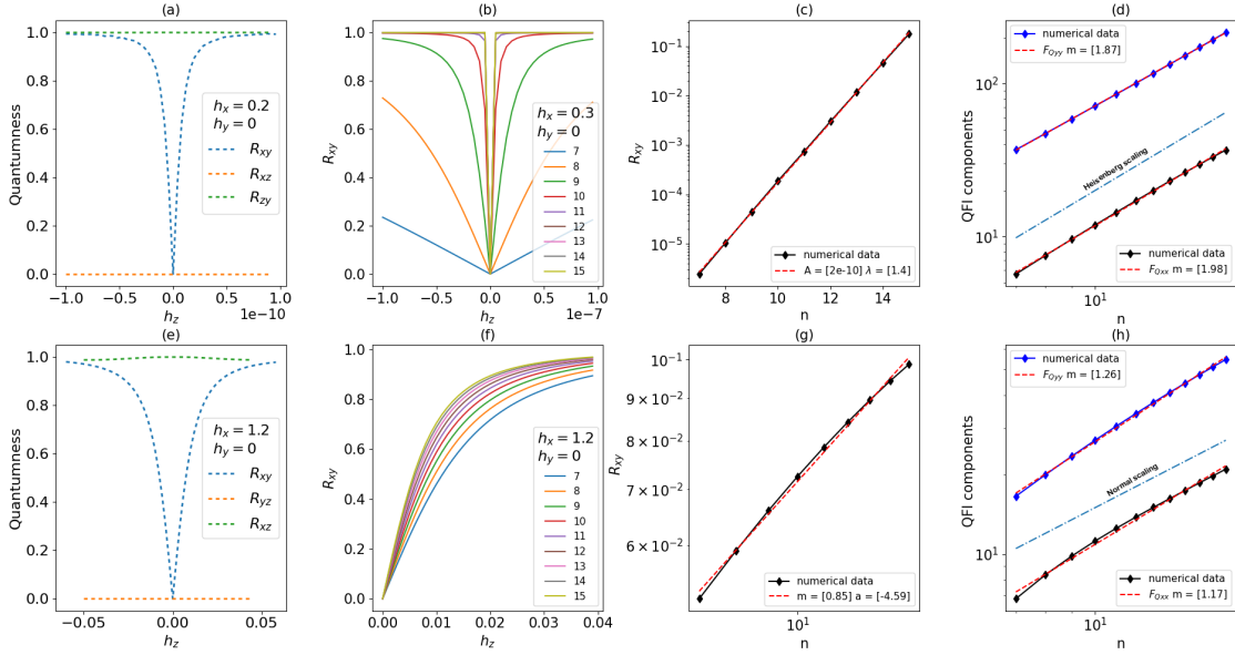
Figure 2: Behaviour of the quantumness and Fisher information in the ordered phase (panels (a-d)) and in the disordered phase (panels (e-h)). In panel (a) and (e) is plotted the quantumness as a function of h_z for h_x = 0.2 and h_x = 1.2 , respectively, with n = 11 . Panel (b) displays the scaling behaviour of the quantumness for h_x = 0.3 as a function of h_z . Panel (c) plots in a semi-log scale the quantumness as a function of n , very close to the first order QPT ( h_x = 0.3 and h_z \sim 10^{-10} ): this shows that R_{xy} decreases abruptly to zero in h_z = 0 , with a rate which scales exponentially with n . Analogously, panel (f) displays the dependence of R_{xy} on h_z and panel (g) its dependence on n close to h_z = 0 and for h_x = 1.2 (log-log scale): the quantumness decreases to zero, but in absence of a first order QPT, it vanishes with a rate which scales as a power-law in n . In the log-log plots in panel (d) and (h) is shown the scaling behaviour of the components of the QFI with respect to the number of spins n . In panel (d) it is shown that for h_x = 0.95 both the components are very close to a Heisenberg scaling. Otherwise, in panel (h) in absence of QPT ( h_x = 1.2 ) both the components are far from a Heisenberg scaling and closer to a normal one. Notice that the fitting parameter m is the slope of the linear fitting, while A and \lambda are the amplitude and the coefficient of the exponential fitting, respectively. In panel (d) and (h), the blue dashed lines are guides for the eye corresponding to Heisenberg and normal scalings, respectively.
