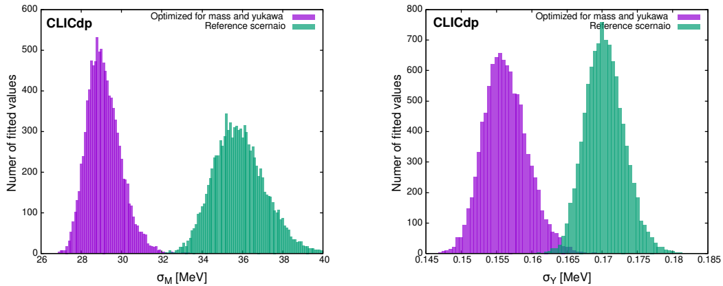
Figure 5: Mass (left) and Yukawa coupling (right) uncertainty distribution in scenario optimised for mass and Yukawa coupling measurement (see Fig. 3), collated with the the reference scenario’s distributions. Figure reproduced from [2].
