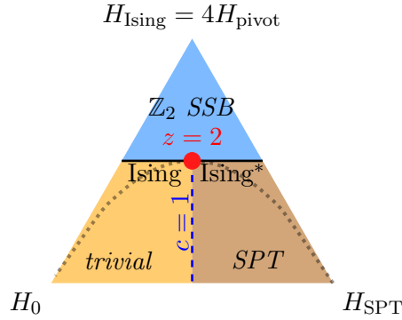
Figure 2: Phase diagram of the 1D cluster SPT transition perturbed by the Ising pivot: Hamiltonian (14) [61–63] plotted in barycentric coordinates. The central vertical axis has an explicit U(1) symmetry generated by H_{\text{pivot}} , which rotates the trivial and SPT phases into one another. This stabilizes a compact boson transition ( c = 1 ) which eventually gaps out upon tuning the filling, making way for a symmetry-breaking phase which satisfies the mutual anomaly between the U(1) symmetry and the \mathbb{Z}_2 \times \mathbb{Z}_2^T symmetry protecting the SPT phase. In the center of the phase diagram, we observe a multicritical point with dynamical critical exponent z = 2 ; this can be perturbed into two topologically distinct symmetry-enriched versions of the Ising criticality [46]. The dotted line is an exactly-solvable frustration-free line which tunes through the multicritical point [61–63]. It is instructive to compare this 1D phase diagram to a 2D analogue in Fig. 6.
