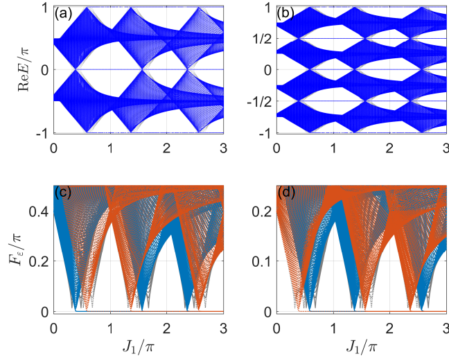
Figure 1: Floquet spectrum E and gap function F_\epsilon of U_{1/2} [Eq. (20)] and U versus J_1 under OBC and PBC. Other system parameters are set as (J_2, \mu, \lambda) = (0.5\pi, 0.4\pi, 0.25) and the length of lattice is L = 400 . (a) and (b) show the values of the real part of E for the parent and square-root models described by U and U_{1/2} under the OBC (PBC) in blue (grey) dots, respectively. The blue solid and red dotted lines denote the gap functions F_0 and F_\pi of U in (c), and the gap functions F_0 (= F_\pi) and F_{\pi/2} of U_{1/2} in (d) under the OBC. Grey solid and dotted lines denote the same gap functions under PBC.
