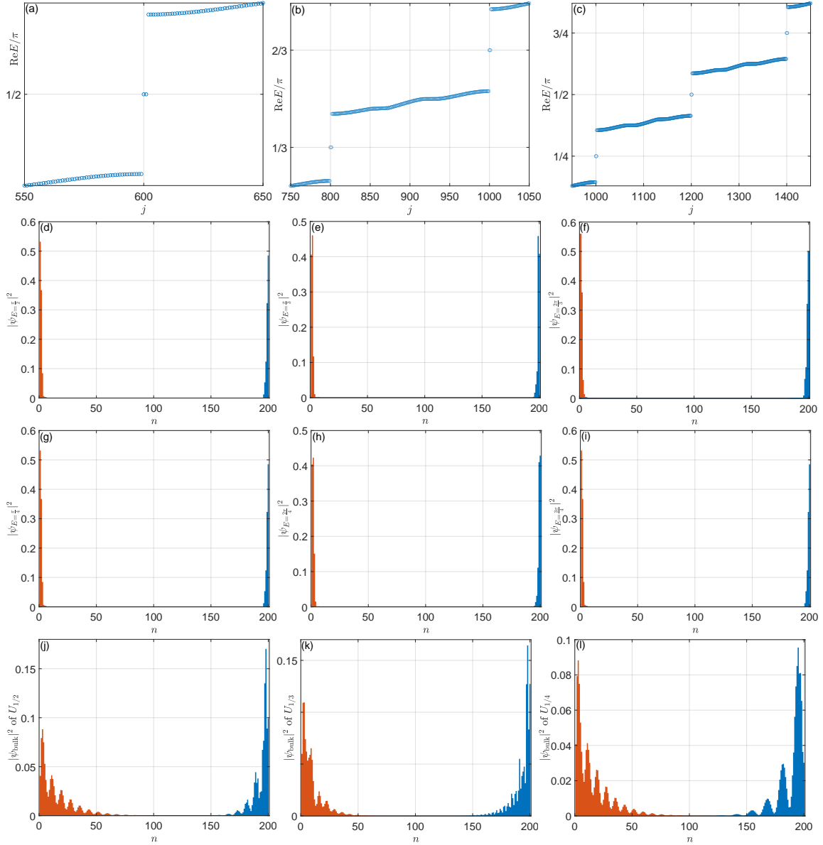
Figure 3: The real part of Floquet spectrum, fractional-quasienergy edge modes and bulk skin modes of the q th-root non-Hermitian FTIs for q = 2, 3, 4 . j and n are state and unit cell indices. System parameters are (J_1, J_2, \mu, \lambda) = (\pi, 0.5\pi, 0.4\pi, 0.25) . The length of lattice is L = 400 . (a), (b) and (c) show the Floquet spectrum of U_{1/2} , U_{1/3} and U_{1/4} , zoomed in around E = \pi/2 , E = (\pi/3, 2\pi/3) and E = (\pi/4, 2\pi/4, 3\pi/4) , respectively. (d) shows the degenerate edge modes of U_{1/2} with E = \pi/2 . (e) and (f) show the degenerate edge modes of U_{1/3} with E = \pi/3 and 2\pi/3 . (g), (h) and (i) show the degenerate edge modes of U_{1/4} with E = \pi/4 , 2\pi/4 and 3\pi/4 . (j), (k) and (l) show three pairs of typical bulk states for U_{1/2} , U_{1/3} and U_{1/4} , respectively, which are piled up around the boundaries and thus represent non-Hermitian Floquet skin modes.
