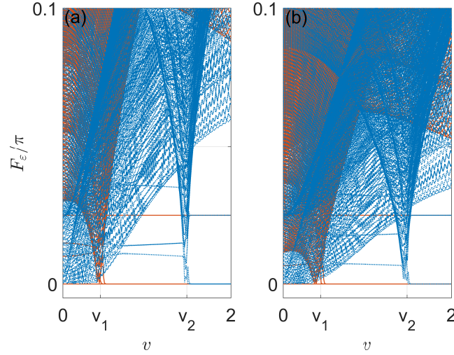
Figure 5: Gap function F_\epsilon of \mathcal{U}_{1/2} [Eq. (26)] and \mathcal{U}_{1/3} [Eq. (27)] versus v . Other system parameters are (J_1, J_2, \Delta, u) = (2.5\pi, 3\pi, 0.05\pi, 0) and the length of lattice is L = 2000 in each spatial dimension. The blue dotted and red solid lines denote the gap functions F_0 (= F_\pi) and F_{\pi/2} of \mathcal{U}_{1/2} in (a), and the gap functions F_{\pi/3} (= F_\pi) and F_{2\pi/3} (= F_0) of \mathcal{U}_{1/3} in (b). v_1 and v_2 are imaginary parts of \mu = u + iv where the spectral gap closes and the number of corner modes change through topological phase transitions, obtained by solving Eq. (28).
