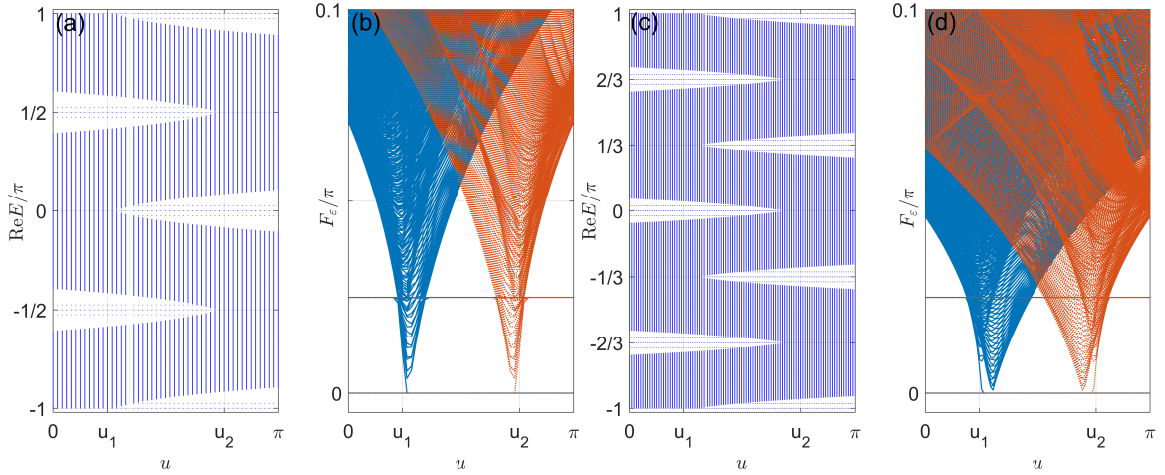
Figure 4: Floquet spectrum E and gap function F_\epsilon of \mathcal{U}_{1/2} [Eq. (26)] and \mathcal{U}_{1/3} [Eq. (27)] versus u . Other system parameters are set as (J_1, J_2, \Delta, \nu) = (0.5\pi, 5\pi, 0.05\pi, 0.5) . The lattice size is L = 2000 along each spatial direction. (a) and (c) show the values of the real part of E for the square- and cubic-root models described by \mathcal{U}_{1/2} and \mathcal{U}_{1/3} , respectively. The blue solid and red dotted lines denote the gap functions F_0 (= F_\pi) and F_{\pi/2} of \mathcal{U}_{1/2} in (b), and the gap functions F_{\pi/3} (= F_\pi) and F_{2\pi/3} (= F_0) of \mathcal{U}_{1/3} in (d). u_1 and u_2 denote critical values of u where the spectral gap closes and the number of corner modes change across the topological phase transition, which are obtained from Eq. (28).
