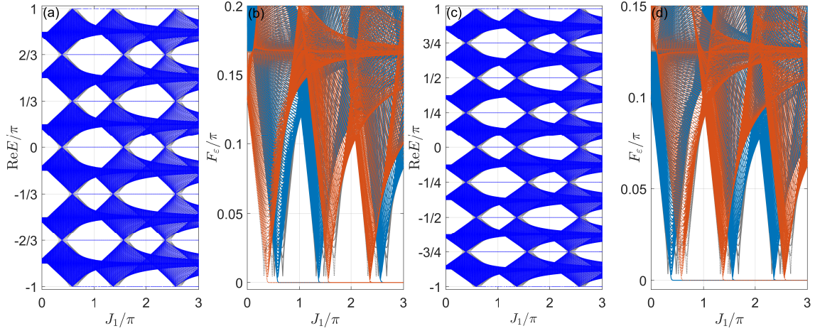
Figure 2: Floquet spectrum E and gap function F_\varepsilon of U_{1/3} [Eq. (21)] and U_{1/4} [obtained following Eqs. (20), (6) and (7)] versus J_1 under both PBC and OBC. Other system parameters and the lattice size are the same as those used in Fig. 1. (a) and (c) show the real parts of E for the cubic- and fourth-root models described by U_{1/3} and U_{1/4} , respectively, under the OBC (blue dots) and PBC (grey dots in the background). The blue solid and red dotted lines denote the gap functions F_{\pi/3} ( = F_\pi ) and F_{2\pi/3} ( = F_0 ) of U_{1/3} in (b), and the gap functions F_{\pi/4} ( = F_{3\pi/4} ) and F_{\pi/2} ( = F_0 = F_\pi ) of U_{1/4} in (d) under the OBC. Corresponding gap functions under the PBC are given by the grey solid and dotted lines in (b) and (d).
