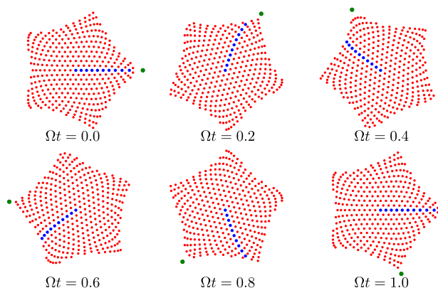
Figure 6. The n = 4 mode. A reference set of vorticities are highlighted in blue, and orbit the center with angular frequency \Omega . A reference deformation peak is indicated by the green dot, and orbits the center with angular velocity \frac{n}{n+1}\Omega .
