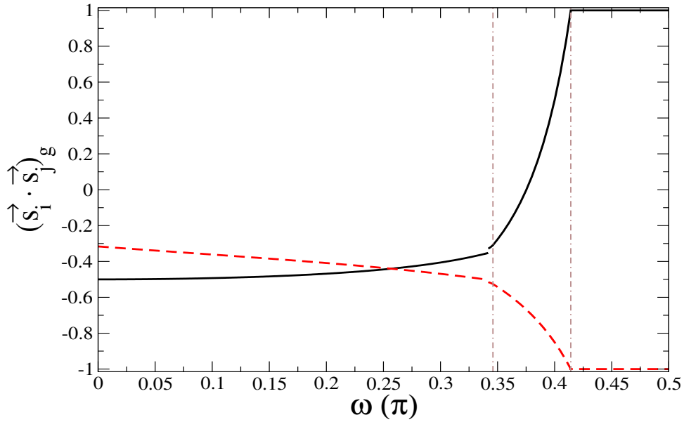
Figure 14: Ground-state nearest-neighbor correlations (\vec{s}_i \cdot \vec{s}_j)_g for Hamiltonian (1) as a function of \omega for the pentakis icosidodecahedron. The (black) solid line corresponds to the icosidodecahedron-edge correlation and the (red) dashed line to the pentagon vertex with the pentagon's center correlation. The corresponding interactions in Hamiltonian (1) are equal to \cos\omega and \sin\omega respectively. The vertical lines show the \omega values where the dimensionality of the MDGS changes from 5 to 4 and then to 1.
