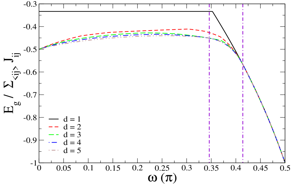
Figure 13: Reduced ground-state energy per bond \frac{E_g}{\sum_{\langle ij \rangle} J_{ij}} for Hamiltonian (1) as a function of \omega for the pentakis icosidodecahedron. The icosidodecahedron-edge interaction equals \cos\omega and the pentagon vertex with the pentagon's center interaction equals \sin\omega . The dimensionality of spin space d ranges from 1 to 5. The vertical lines show the \omega values where the dimensionality of the MDGS changes from 5 to 4 and then to 1.
