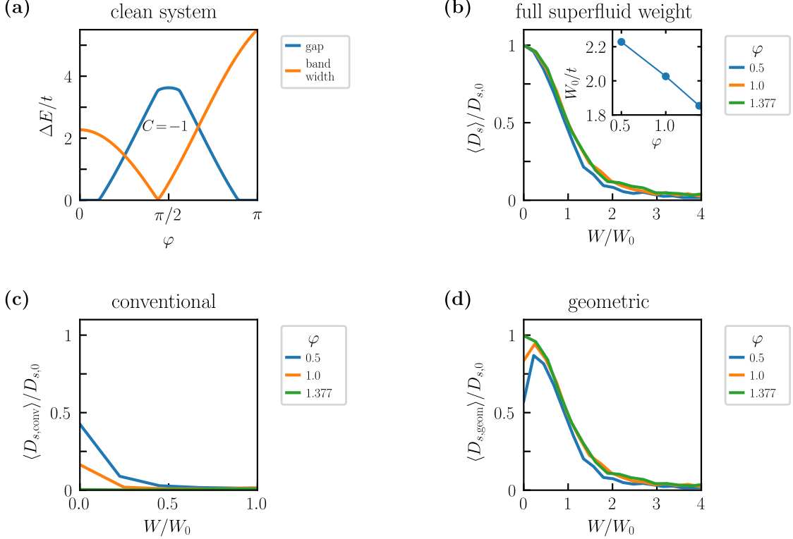
FIG. S4. Properties of the extended Kane-Mele model as a function of the NNN hopping phase \varphi for U = 3t , T = T_{c,0}/100 , and \bar{\nu} = 1/2 : (a) Evolution of the energy gap and the bandwidth of the lower band. The band has optimal flatness at \varphi_{\text{opt}} = 1.377 . We also indicate the Chern number of the lower spin-up band where the gap is nonzero. Full superfluid weight (b), conventional contribution (c), and geometric contribution (d) as a function of disorder W for various fixed NNN hopping phases \varphi . The inset in (b) shows the disorder scale W_0 as a function of \varphi .
