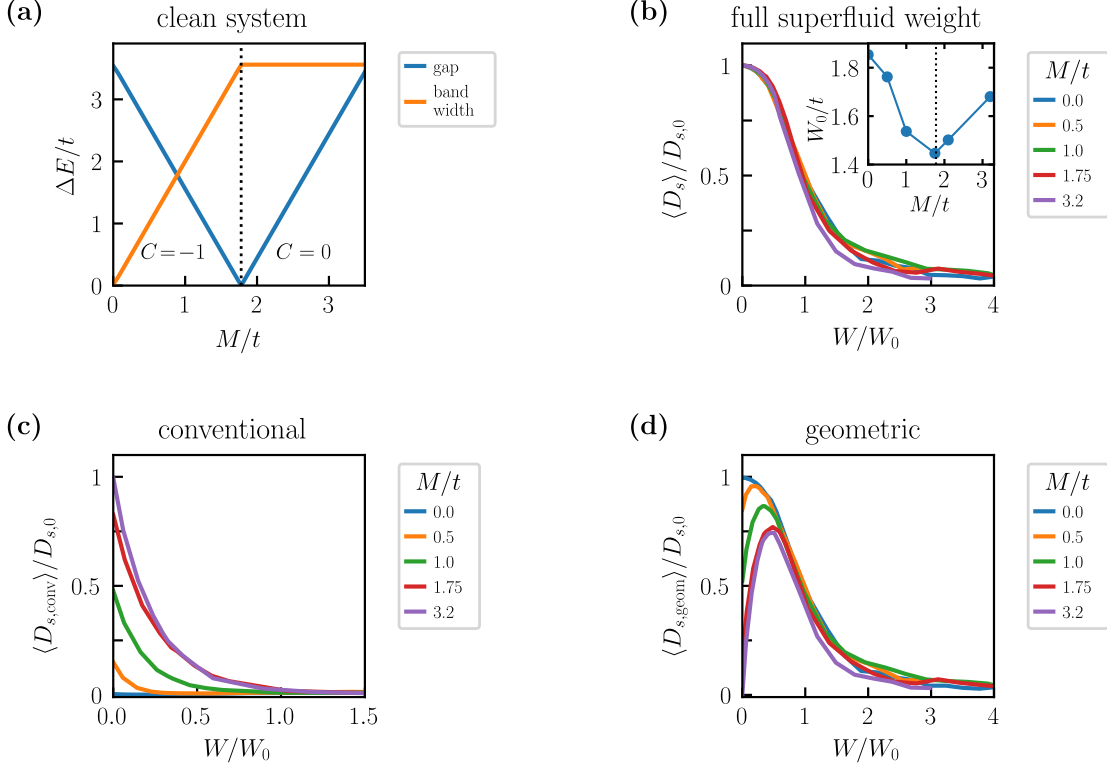
FIG. S3. Properties of the extended Kane-Mele model as a function of the staggered onsite potential M for U = 3t , T = T_{c,0}/100 , and \bar{\nu} = 1/2 : (a) Evolution of the energy gap and the bandwidth of the lower band. We also indicate the Chern number of the lower spin-up band on the two sides of the topological transition. Full superfluid weight (b), conventional contribution (c), and geometric contribution (d) as a function of disorder W for various values of M . The inset in (b) shows the disorder scale W_0 as a function M .
