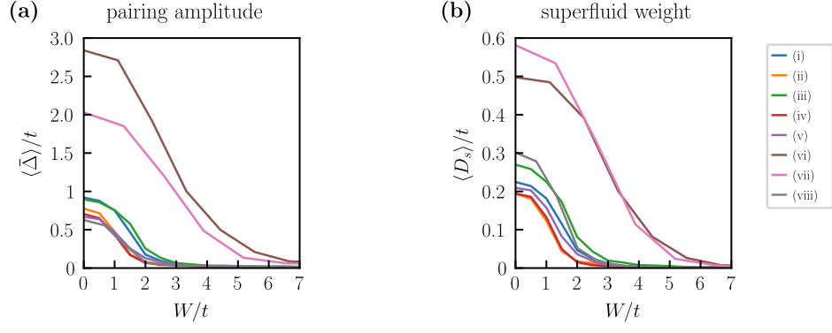
FIG. S9. Disorder-induced suppression of the pairing amplitude and the superfluid weight across a variety of lattice models corresponding to Fig. 1 of the main text: (i)-(v) topological and trivial extended Kane-Mele models, (vi)-(viii) trivial single-band models. The ensemble averages of (a) the spatial average of the pairing amplitude \bar{\Delta} and (b) the superfluid weight D_s are shown as a function of the disorder strength W . In contrast to Fig. 1 of the main text, we here show the unscaled quantities in units of the nearest-neighbor hopping amplitude t of the respective model.
