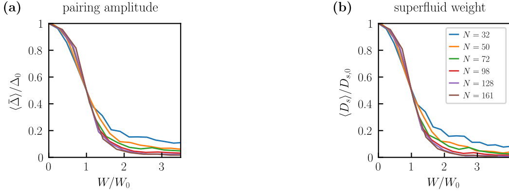
FIG. S6. Disorder-induced suppression of the pairing amplitude and the superfluid weight for different cluster sizes. We show results for the extended Kane-Mele model with flat lower band and U = 3t , T = T_{c,0}/100 , and \bar{\nu} = 1/2 .
