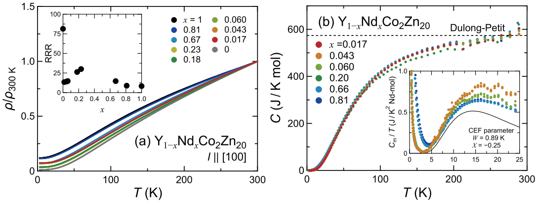
Figure 1: (a) Normalized electrical resistivity \rho(T)/\rho(300 \text{ K}) versus temperature T of \text{Y}_{1-x}\text{Nd}_x\text{Co}_2\text{Zn}_{20} for 0 \leq x \leq 1 . The \rho(T) data for x = 1 are from [8]. The inset shows the residual resistivity ratio as \text{RRR} = \rho(300 \text{ K})/\rho(3 \text{ K}) . (b) Specific heat C versus T of \text{Y}_{1-x}\text{Nd}_x\text{Co}_2\text{Zn}_{20} for 0.017 \leq x \leq 0.81 . The dashed line is the Dulong-Petit value of 573.7 \text{ J/K mol}^{-1} . The inset shows the magnetic specific heat divided by temperature C_m/T for x = 0.043, 0.060, 0.66, and 0.81 . The solid line represents the CEF calculation.
