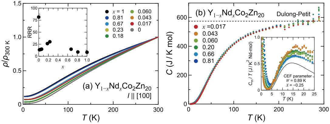
Figure 1: (a) Normalized electrical resistivity \rho(T)/\rho(300\text{ K}) versus temperature T of \text{Y}_{1-x}\text{Nd}_x\text{Co}_2\text{Zn}_{20} for 0 \leq x \leq 1 . The \rho(T) data for x = 1 are from [8]. The inset shows the residual resistivity ratio as \text{RRR} = \rho(300\text{ K})/\rho(3\text{ K}) . (b) Specific heat C versus T of \text{Y}_{1-x}\text{Nd}_x\text{Co}_2\text{Zn}_{20} for 0.017 \leq x \leq 0.81 . The dashed line is the Dulong-Petit value of 573.7\text{ J/K mol}^{-1} . The inset shows the magnetic specific heat divided by temperature C_m/T for x = 0.043, 0.060, 0.66, and 0.81 . The solid line represents the CEF calculation.
