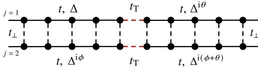
Figure 1: Schematic illustration of the junction system consisting of two Kitaev ladders. Note that the superconducting pair potential \Delta is only assumed within each chain. Here, two superconducting phase differences are assumed; \theta is the Josephson phase difference across the junction, and \phi is the additional inter-chain phase difference.
