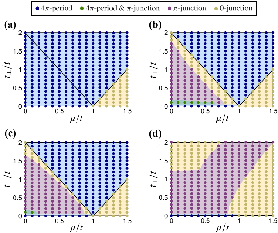
Figure 4: The correlation between the types of E_J(\theta) on the phase diagram of the Kitaev ladder for (a) \phi = 0 , (b) \phi = \pi/3 , (c) \phi = 2\pi/3 , and (d) \phi = \pi . Solid lines represent the boundary of the topological phase.
