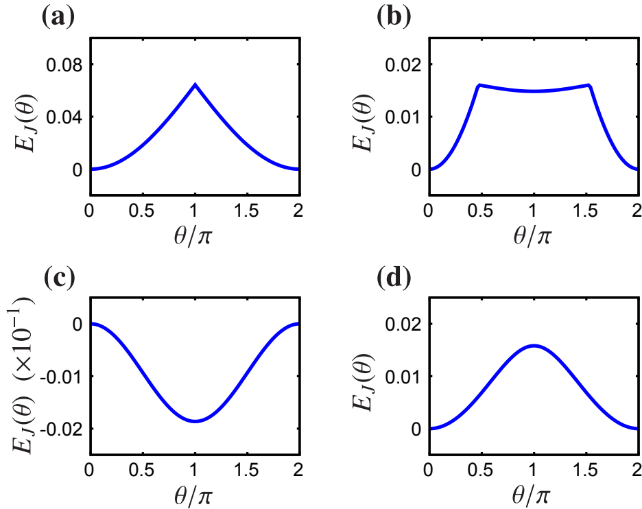
Figure 2: The Josephson energy-phase relation E_J(\theta) of the ladder junction model when (a) t_\perp/t = 0 , (b) t_\perp/t = 0.1 , (c) t_\perp/t = 0.3 , (d) t_\perp/t = 1.0 .
