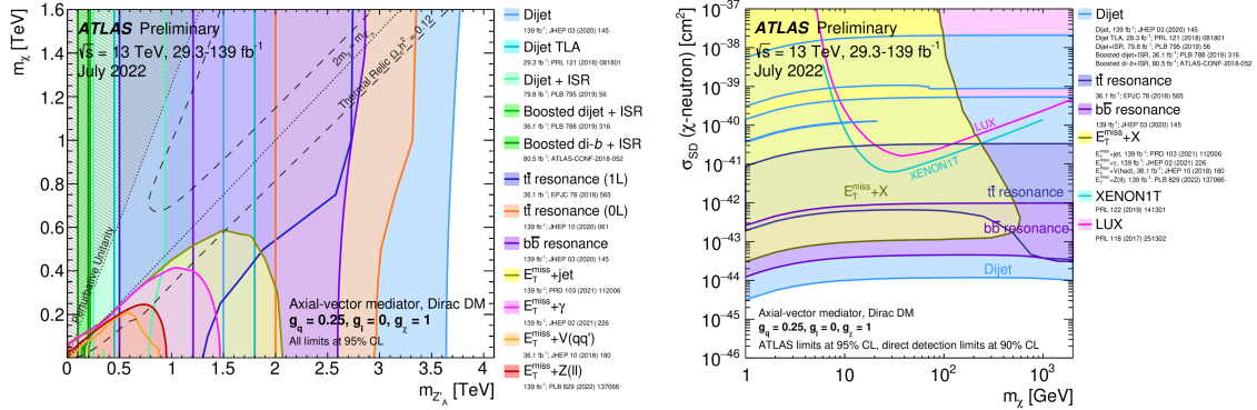
Figure 4: (Left) Exclusion limits on the \{m_\chi, M_{med}\} plane (axial-vector) mediator. (Right) Exclusion limits expressed in terms of equivalent WIMP-neutron cross-section as a function of m_\chi [4].
