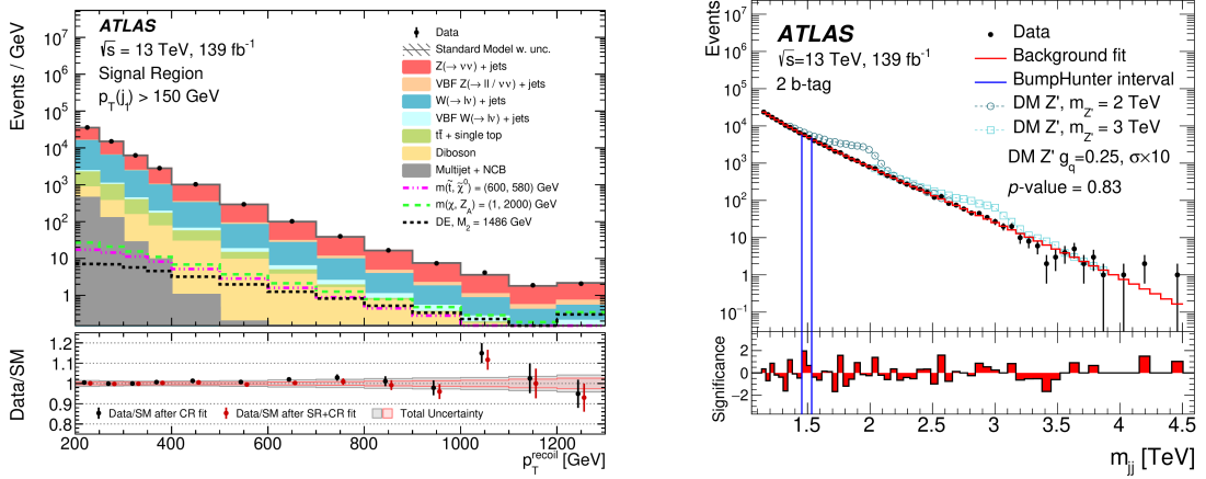
Figure 2: Distribution of (left) p_T^{\text{recoil}} for \cancel{E}_T + \text{jet} events and (right) m_{jj} for di-jets.
