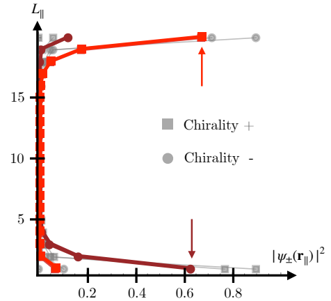
FIG. 10. Fractional nature of the NH higher-order flux skin effect. Eigenstates of the chiral symmetry in the EHH appear with zero net-chirality per surface in the absence of a magnetic flux \phi . Introducing a flux defect with \phi = \pi leads to additional contributions to top and bottom surface (depicted in red), having opposite chirality. Panel is generated for a model of size 20 \times 20 \times 20 unit cells in NH class A with additional pseudo-inversion symmetry (see App. E 2 b).
