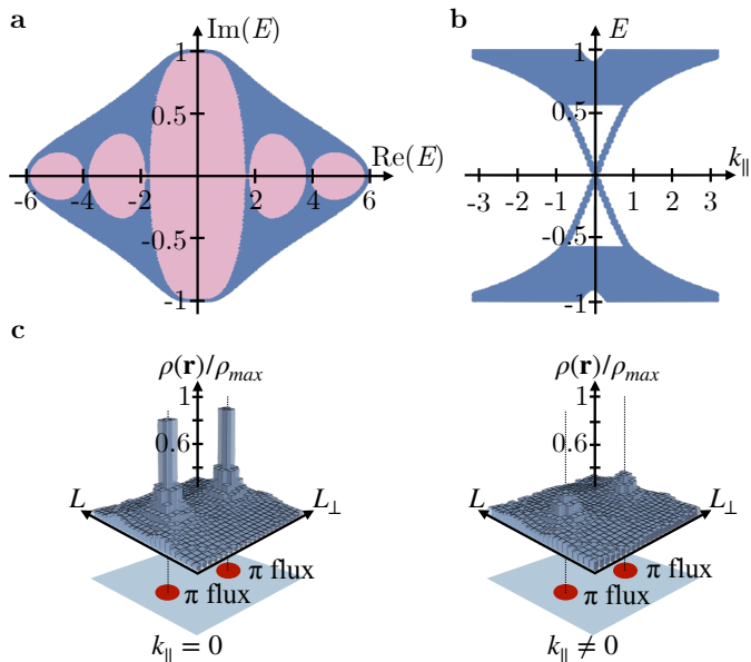
FIG. 4. NH flux spectral jump in 3D. a Spectrum in the complex energy plane under PBC (blue) and SIBC in presence of \pi -flux tubes (blue and red) for a model exhibiting nontrivial point gap topology in NH class \text{AII}^{\dagger} [Eq. (E7)]. Flux-localized states fill the SIBC spectral point gap at a single momentum k_{\parallel} = 0 along the flux tube. b At this momentum, the EHH spectrum exhibits a helical crossing at zero energy for any E_0 located in the central point gap. c The flux spectral jump localizes an extensive number of eigenmodes at the flux tubes, indicated by two peaks of the summed density \rho(\mathbf{r}) = \sum_{\alpha,i} |\langle \mathbf{r}_i | \psi_{\alpha} \rangle|^2 , where \alpha ranges over all eigenstates \psi_{\alpha} of the Hamiltonian with flux defect, \mathbf{r} denotes the lattice site and the summation i runs over sublattice degrees of freedom.
