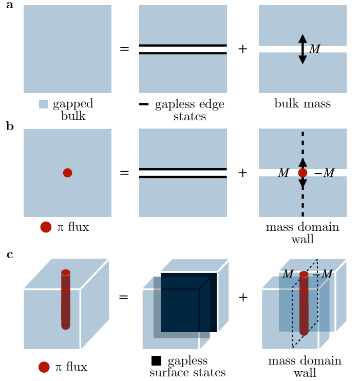
FIG. 7. Dirac theory of flux response. a The gapped bulk of a topological insulator can be viewed as a combination of two subsystems, whose edge states are gapped by a bulk mass term. b Bound states localized at \pi -fluxes in Hermitian insulators can be viewed as domain wall bound states of the Dirac mass associated with a pair of edge states [14]. c In 3D, \pi -fluxes similarly bind 1D states.
