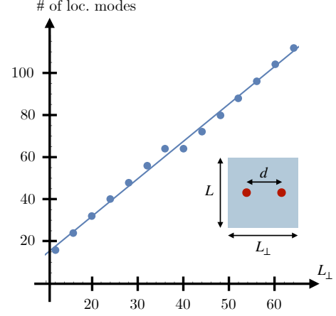
FIG. 8. Scaling analysis for the NH flux skin effect. The number of modes with more than 70% localization at the flux cores scales linearly with the extent of the system along the direction connecting the two flux cores L_{\perp} . The separation between the flux cores d is held fixed. The fit is given by \# = -3.81538 + 1.78462 L_{\perp} , using a model in NH class AII † [Eq. (E1)].
