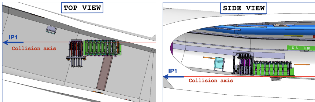
Figure 2: Side and top views of the SND@LHC detector in the TI18 tunnel [7].
