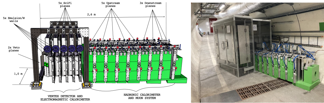
Figure 1: Detector layout (left) and picture of the detector installed in TI18 (right).
