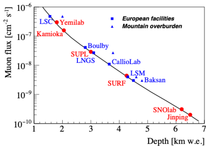
Figure 3: Muons flux in underground laboratories. The solid black line shows the muon flux as a function of depth for a flat overburden. For laboratories under a mountain the muon flux has an angular dependence. In the figure for these cases a maximum overburden is shown. This is greater than the overburden predicted under a flat surface. For comparison all laboratories have been overlaid to the solid line.
