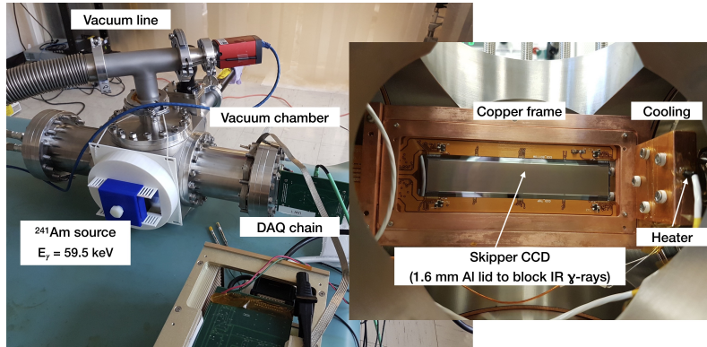
Figure 1: Experimental setup during the Compton data taking. The blue box fixed on the flange of the vacuum chamber contains the ^{241}\text{Am} source with Al plate blocking low energy \gamma -rays.
