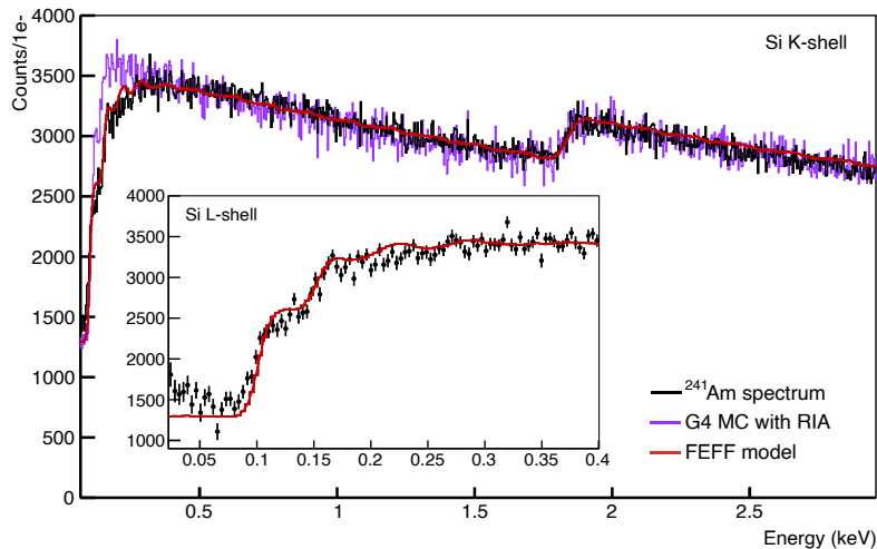
Figure 2: The measured ^{241}\text{Am} Compton spectrum (black) with the GEANT4 simulated spectrum based on the relativistic impulse approximation (purple) and the FEFF calculation (red). The inset shows the data comparison to the FEFF prediction in the L-shell energy range.
