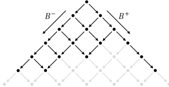
Figure 15: One example of 3d CCA representation where the black dots representing the operators of this representation fitting in the 2d grid shown in gray.
