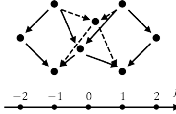
Figure 16: The representation in (C.4). The points represent the operators and the axis labels their spin. This is exactly the second part in the rank-3 tensor representation shown in Figure 19.
