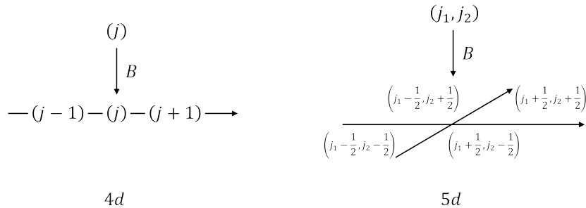
Figure 14: Since the SO(4) representations are labeled by (j_1, j_2) , which form a 2-dimensional structure, the general net structure of 5d CCA representation should be three dimensional.
