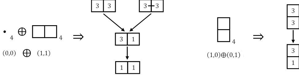
Figure 13: The rank-2 tensor representation of SO(4) and their Inonu-Wigner contraction of the Carrollian limit.
