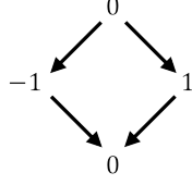
Figure 20: The representation behaves similar to (0) \rightarrow (1) \rightarrow (0) representation in 4d .
