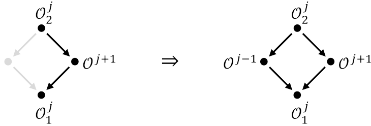
Figure 18: The commutation relation [B^+, B^-] = 0 completes the folded-line structure to a diamond structure.
