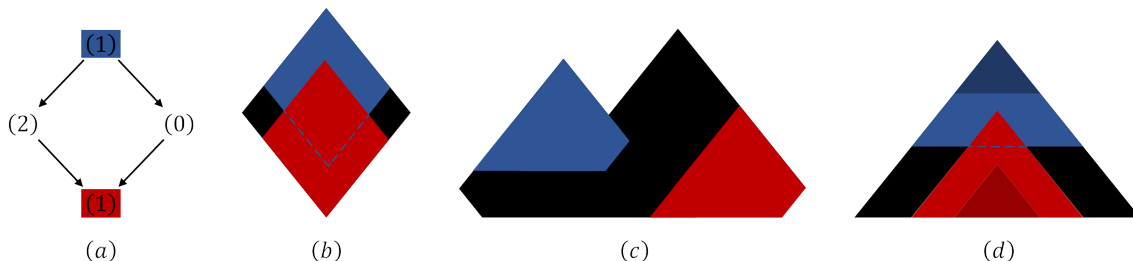
Figure 11: Some examples of self-symmetric representations.
