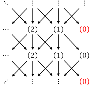
Figure 12: An example with two ending (0) sub-sectors (red ones), and there is only one (1) sub-sector links to each one. Noticing the middle (0) sub-sector is not an ending.
