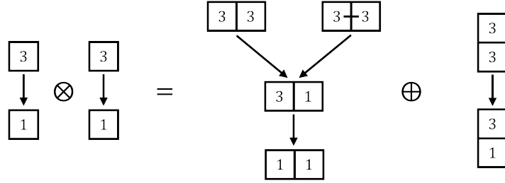
Figure 3: The rank-2 tensor representation of CCA.
