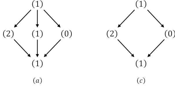
Figure 10: Representation (a) and (c) in Figure 6 repeated here.
