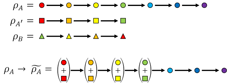
Figure 9: The representation \rho_{A'} have the same structure as the leading parts of the representation \rho_A , and \rho_{A'} = \rho_B^{\text{dual}} . The basis change we consider here is \rho_A \rightarrow \rho_A + c\rho_{A'} .
