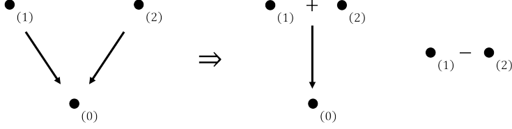
Figure 7: Basis change for a 2d GCA representation to chain representations.
