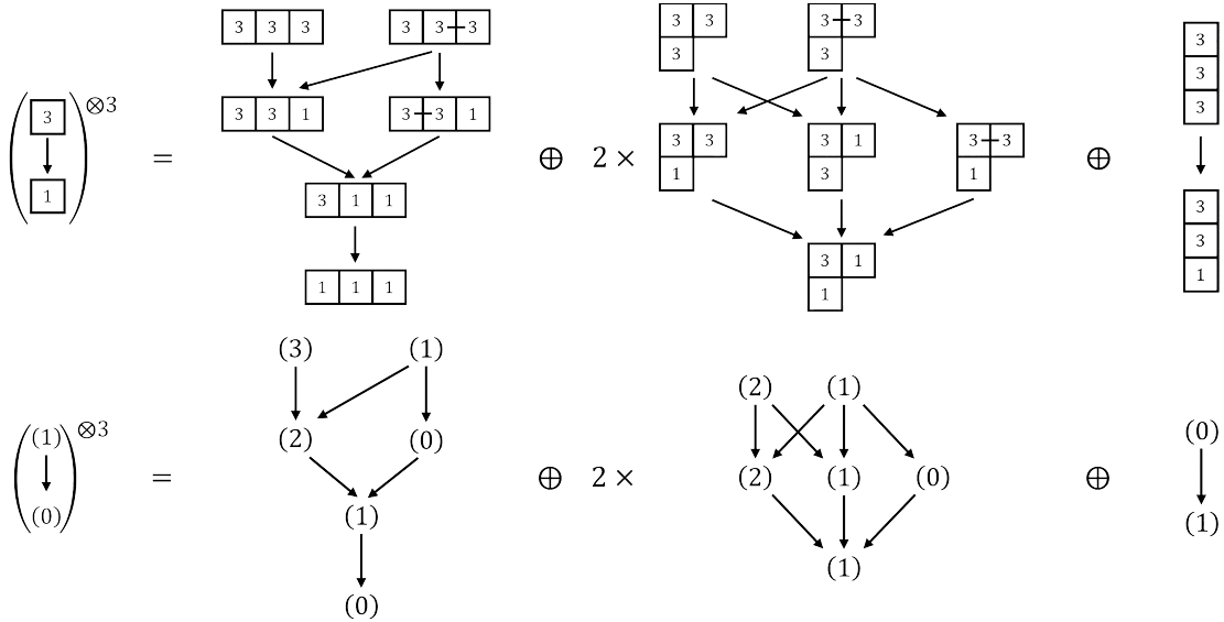
Figure 4: The rank-3 tensor representation of CCA.
