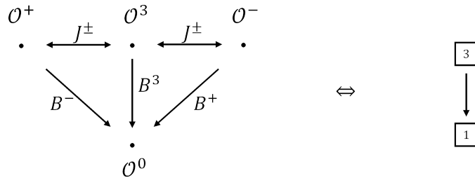
Figure 2: The vector representation of CCA rotation group. The right side is the corresponding Young tableau notation, where \boxed{3} represents a spacial SO(3) index forming the spin-1 SO(3) representation, \boxed{1} represents the temporal index forming the spin-0 SO(3) representation, and the arrow represents the action of B^i generators.
