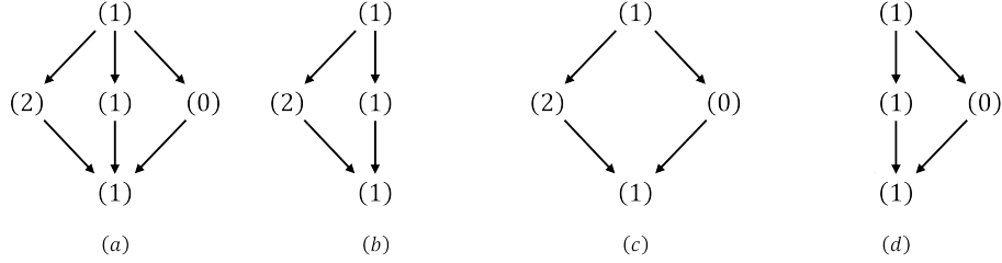
Figure 6: All the four net representations are legal although the middle level of the representations are different.
