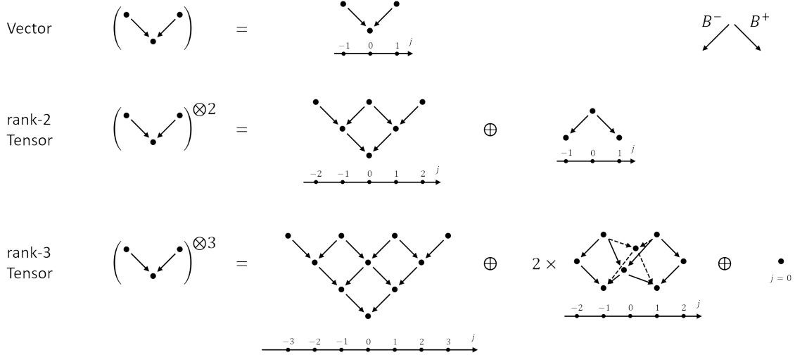
Figure 19: The first three lowest-rank tensor representations. The axes beneath every irreducible representations show the spins, and the arrows label the connection by B generators.
