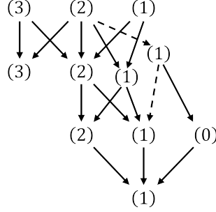
Figure 17: The 45-dimensional indecomposable rank-4 tensor representation of 4d CCA rotations. There are two (1) sectors at order 3 that can not be diagonalized. The rank-4 tensor representation appears in the decomposition of the tensor product: ((3) \rightarrow (1))^{\otimes 4} = [35] \oplus 3 \times [45] \oplus 2 \times [20] \oplus 3 \times [15] \oplus [1] , where [dim] represents a dim -dimensional representation.
