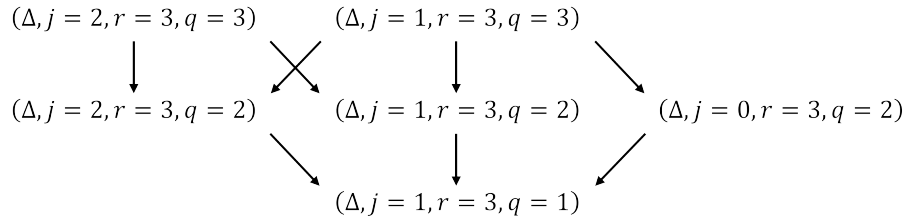
Figure 8: The second part of the rank-3 tensor representation of CCA consists of a \{\Delta, r = 3\} representation.
