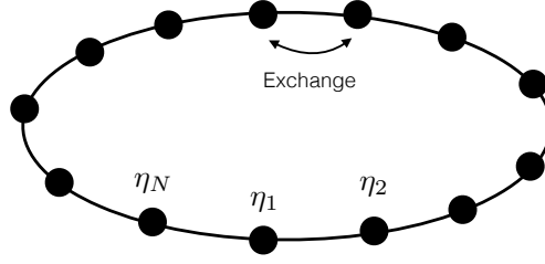
Figure 1: A schematic diagram of the HCVE model. Each site contains some variable \eta_i which are called ‘volume’. These variables are subjected to harmonic potential V(\eta) = \frac{k_0\eta^2}{2} at each lattice site. In addition to the deterministic evolution, ‘volume’ variables on successive sites are exchanged with rate \gamma .
