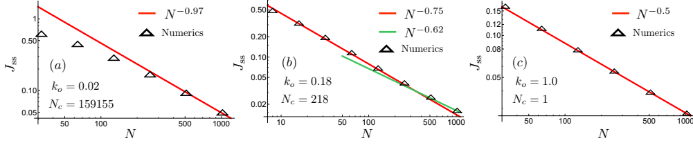
Figure 3: Plot of J_{ss} vs. N for \gamma = 1 and different values of k_o i.e. for different values of N_c as given by Eq. (69). The symbols are obtained by solving the equations of the two-point correlations \langle \eta_i \eta_j \rangle_{P_{ss}} in NESS numerically for different N . In (a) we observe diffusive scaling as one has N \ll N_c = 159155 . In (b), the value of N_c = 218 . We observe a change in the exponent of the system size scaling from 0.75 to 0.62. In principle, one should observe a crossover from diffusive (exponent 1) to anomalous (exponent 0.5) behaviour. For that one needs to have a sufficiently large N_c so that one has sufficiently large N even for N < N_c to observe the true diffusive scaling and then one should be able to evaluate stationary currents J_{ss} for N much large than N_c to observe the true anomalous scaling. Numerically this is very hard to achieve. Instead, in (c) we choose k_o = 1.0 so that one observes only the anomalous scaling because N_c = 1 .
