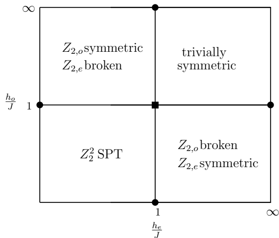
Figure 5. The phase diagram of the model (51) with \mathbb{Z}_2 \times \mathbb{Z}_2 symmetry. The black square locates the critical point described by free boson conformal field theory. All other transition between two gapped phase are described by the Ising conformal field theory.
