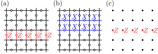
Figure 4. Examples of (a) a U^Z operator, (b) a U^X operator, and (c) an \Omega^Z operator of the bulk model in Eq. 9, all viewed from z direction.
