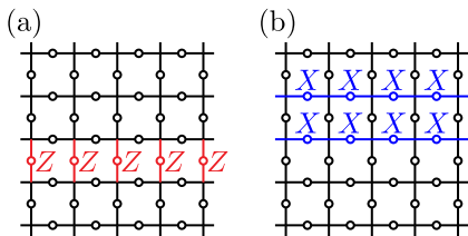
Figure 1. Nonlocal symmetry generators of the model in Eq. 3. U_1^Z is illustrated in (a). U_2^Z is similar but extended along the vertical direction. (b) is an example of an X -type symmetry generator.
