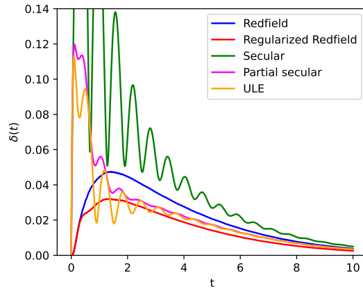
Figure 3: Distance from the exact dynamics as represented by the quantity \delta(t) , defined in (44), using the Hilbert-Schmidt norm. Here \omega_1 = 10 , \omega_2 = 20 , \omega_0 = 15 , \gamma_1 = \gamma_2 = 1 , and \mu = 20 . The various master equations are chosen as in Fig. 2. Similar results are obtained with different choices of parameters, while still remaining in the Markovian regime.
