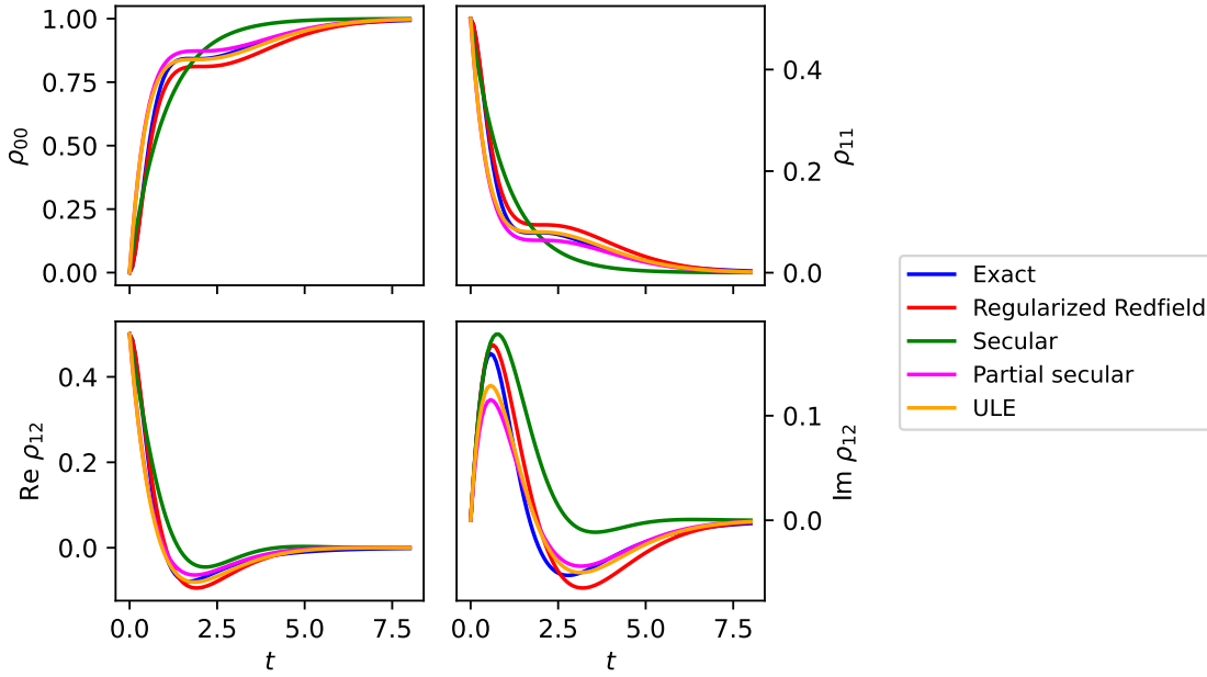
Figure 2: Temporal evolution of the density matrix elements starting from the pure state |\psi_0\rangle = (|1\rangle + |2\rangle)/\sqrt{2} . The label “Regularized Redfield” refers to the proposal of the present paper. The partial secular case (cf. (14)) is obtained by finding the smallest coarse-graining time that guarantees positivity of the Kossakowski matrix. The label “ULE” refers to the “universal Lindblad equation” described in Ref. [22] (also, cf. (16)). Here \omega_1 = 1 , \omega_2 = 2 , \omega_0 = 1.5 , \gamma_1 = \gamma_2 = 1 , and \mu = 4 .
